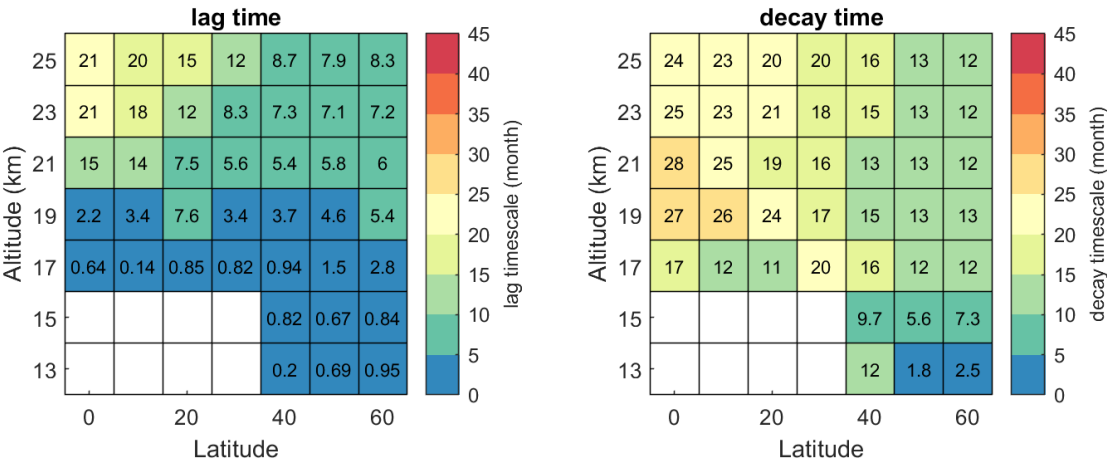
350 Figure 5: Best fit lag and decay timescales from application of the lagged-decay model (Eq. 5) to the passive tracer pulse experiments for June injections as a function of injection latitude and altitude.
