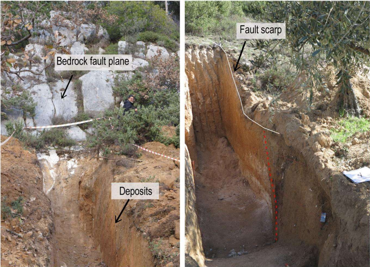
207 208 Figure 4. Field pictures of trench TA (left) and trench TB (right).
