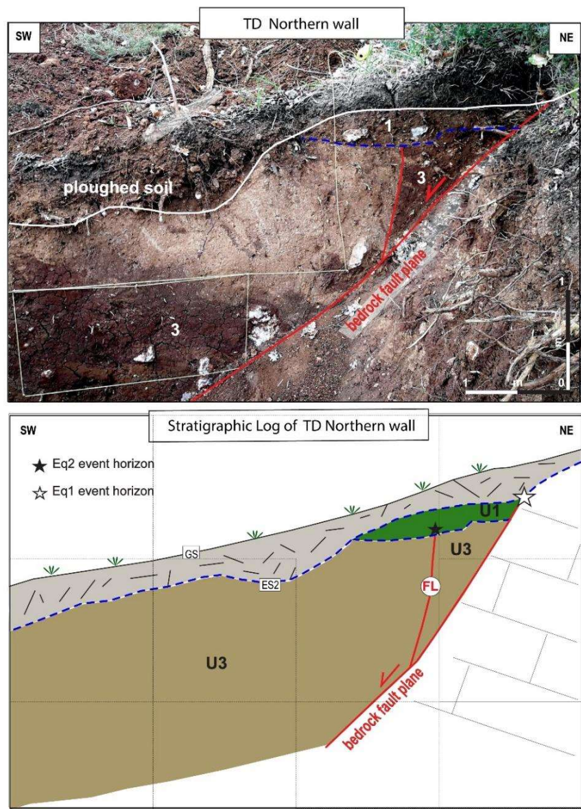
Figure 11. Picture of the northern wall of trench TD (upper panel) and related stratigraphic log scheme (lower panel); red lines mark the fault planes. The stratigraphic units are the same as described in Fig. 9. ES: erosional Surface; GS: Ground Surface.
