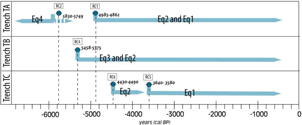
464 465 Figure 12. Chronogram of the surface-rupture events identified from within the TA-TB-TC trenches. Each radiocarbon 466 sample is indicated by the blue circle, labelled, and reported with its 2σ calibrated interval. Horizontal blue arrows point to 467 the assumed paleo event age of occurrence as deduced from the post-quem samples age (see text for further details).
