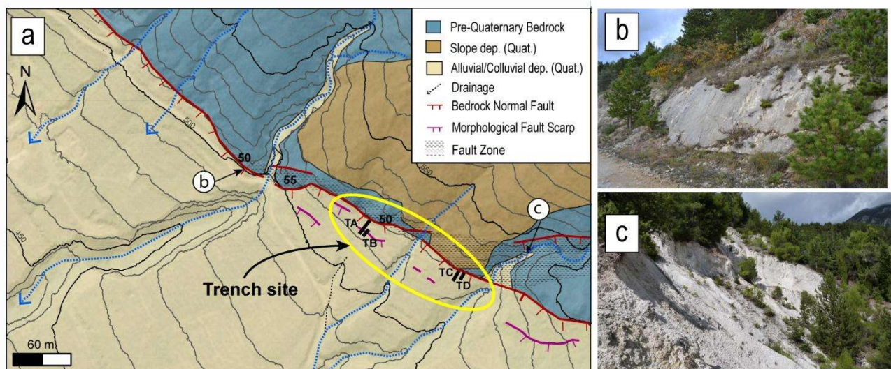
Figure 3. a) Simplified geological map of the study area. The four trenches are indicated by the black segments within the yellow ellipse. The contour lines are 10 metres each, and the field picture's location is indicated. B) Field picture of the cataclasite at the Roccasale fault main slip plane outcropping along the road. C) Field picture of the Roccasale cataclastic fault zone.
