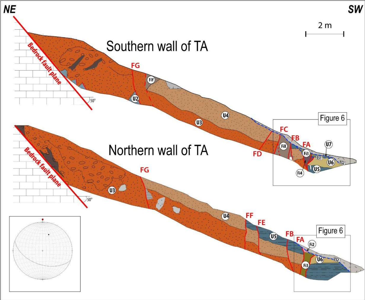
226 227 Figure 5. Stratigraphic sketch logs of the Trench TA's southern and northern walls. The northern wall log is mirrored (to 228 its actual appearance) to highlight the correspondence between the two walls. The stereo plot indicates the bedrock fault 229 plane measured at the top end of the trench (200/50). Units and faults, marked by red lines, are labelled in the figure.
