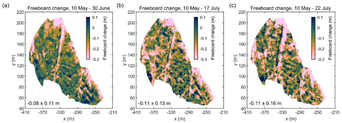
Figure RC4-2: Snow/SSL freeboard change between 10 May and 30 June (a), 17 July (b), and 22 July (c).
