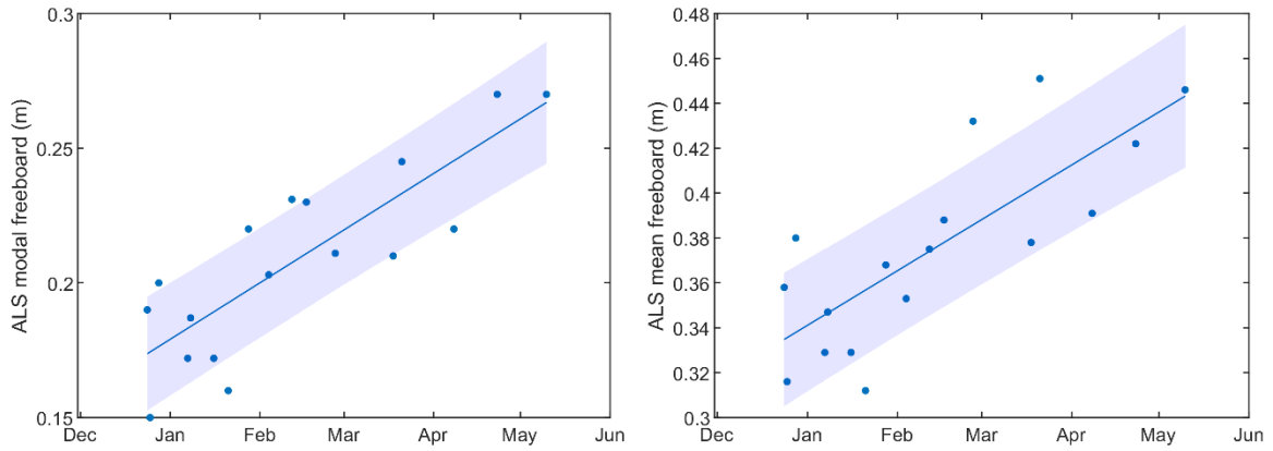
Figure RC4-1: Modal (left) and mean (right) freeboard for full ALS surveys during the freezing season.
