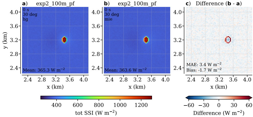
Figure A1. The effect of phase function choice in the cloud_gap case with solar zenith angle set to 30^\circ . Subplot (a) shows the total SSI using Henyey-Greenstein (HG) and (b) using Mie look-up tables. The difference in (c) shows the increase in SSI at the project cloud gap edge and slight decrease just around it, highlighting that Mie resolves the narrow forward scattering peak whereas HG is more diffuse.
