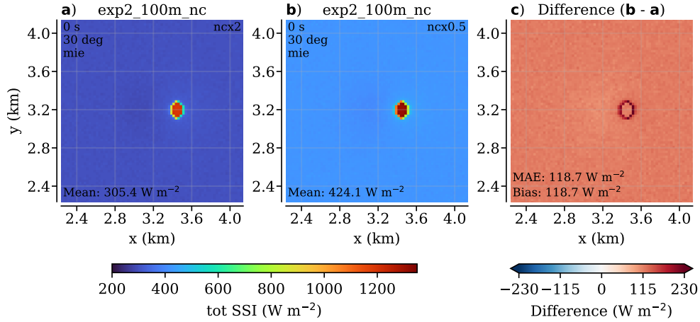
Figure A4. The effect of changes in droplet number concentration ( nc ) in the cloud gap case with solar zenith set to 30^\circ . All simulations use the Mie phase function. The nc is doubled ( nc200 ncx2 ) and halved ( nc50 nc0.5 ) relative to the standard simulations (200e6 and 50e6) and shown in respectively (a) and (b). The rest of the layout is the same as Figure A1. The increased effective radii in (b) compared to (a) result in a lower optical thickness, brightening the whole scene shown in (c).
