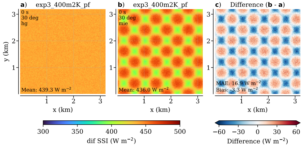
Figure A2. The effect of phase function choice in the checkerboard case with solar zenith set to 30^\circ . Same layout as Figure A1, but for diffuse SSI.
