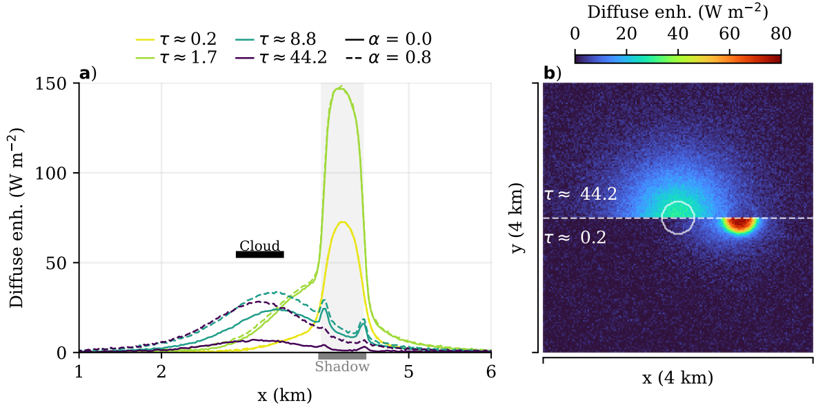
Figure 8. From forward escape to downward escape. A cloud disk at 1 km altitude with 25 m in depth and a 500 m diameter scatters radiation coming in at a zenith angle of 45°. Diffuse SSI enhancement is calculated relative to clear-sky diffuse values. The lines in (a) are averaged over the middle 400 m in the y-direction, whereas (b) shows the 2D surface field. The circle in the centre of (b) marks the edge of the cloud disk.
