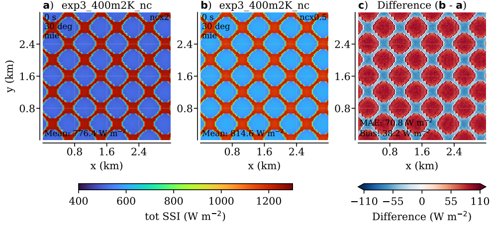
Figure A5. The effect of changes in droplet number concentration (nc) in the checkerboard case with solar zenith set to 30^\circ . Same experiment and plot layout as Figure A5. The increased effective radii in (b) compared to (a) result in a lower optical thickness and less diffusive forward scattering, brightening the projected shadows and darkening the sunlit areas, shown in (c).
