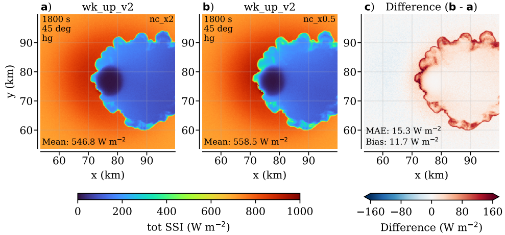
Figure A6. The effect of changes in droplet number concentration (nc) in the shear-free cumulonimbus case with solar zenith set to 45^\circ . Here, we use the Henyey-Greenstein phase function. The nc for both ice and water are doubled and halved relative to the standard simulations (200e6 and 50e6 for water, 2e5 and 5e4 for ice). Same layout as Figure A5. The increased effective radii in (b) compared to (a) result in a lower optical thickness and less diffusive forward scattering, brightening the projected shadows and darkening the sunlit areas, shown in (c).
