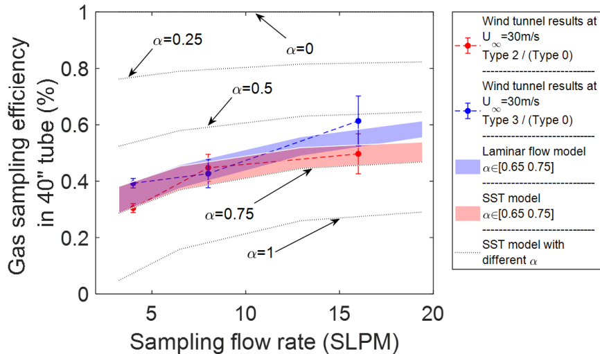
Figure 4. Comparison of different types of sampling tubes and the gas transmission efficiency: Comparison of the gas sampling efficiency measured along 40" (~1 m) of a straight sampling tube with simulation results that vary the sticking coefficient, \alpha_i . The error bar is uncertainty of the data which follows the description of propagation analysis in the supplement.
