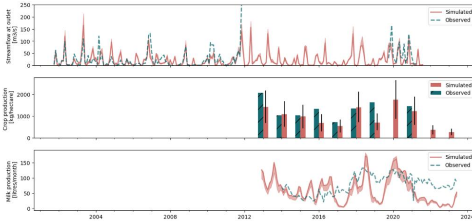
335 Figure 4: Observed and simulated timeseries of streamflow at the outlet of the catchment ( m^3/s ), crop production (kg/hectare), and milk production (litres/month). The uncertainty ranges indicate the 10 th and 90 th percentile, resulting from the different parameter sets of the best ten performing runs.
