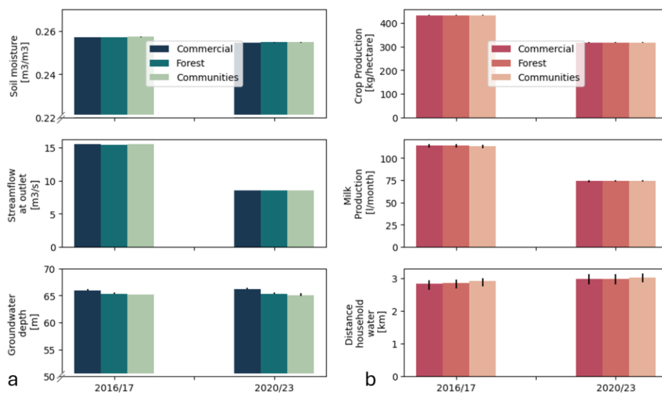
Figure 5: Average of drought hazard (a) and impact (b) over the four sub-catchments for two drought periods in the three scenarios. The error bars show the 25 th and 75 th percentile of the runs.
