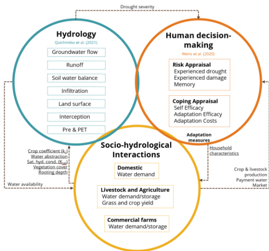
110 Figure 2: ADOPT-AP modelling framework, consisting of three modules; hydrology, human decision-making, and socio-hydrological interactions.
