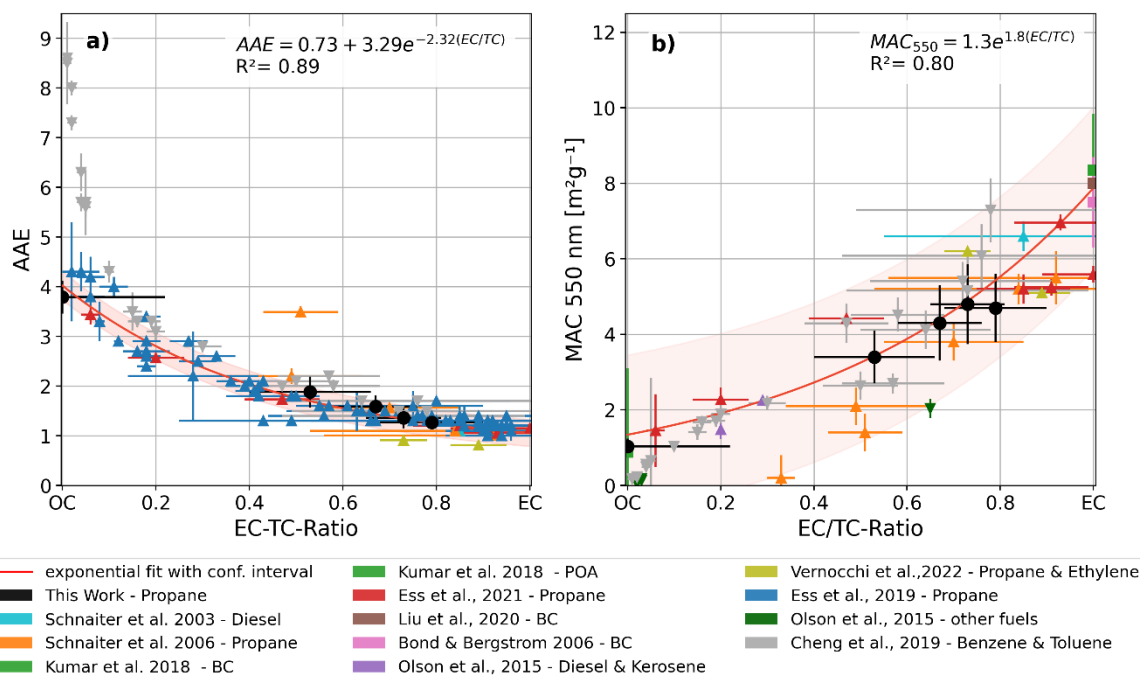
Figure 6 Compositional dependent absorption mass absorption cross sections (MAC, right panel) and its spectral variability represented by the absorption Ångström exponents (AAE, left panel). The MAC data obtained in the present study at 550 nm (black points) are combined with observations from past literature studies and put in relation to the EC/TC soot content. Data are fitted with the equation: y = a + b * e^{(c*EC/TC)} . Due to their fuel type, the soot produced by Cheng et al. (2019) (grey) and the other fuels from Olson et al. (2015), as well as values for pure BC and primary organic aerosols (POA) (Bond and Bergstrom, 2006; Kumar et al., 2018; Liu et al., 2020b), are not considered in the fits. In order to account for error bars in the fit an arbitrary minimal error of 10^{-3} was applied for EC/TC-ratios when these were not provided in their respective source studies. Any other uncertainty in the retrieved values was propagated according to the used calculation. The resulting equations for the absorbing properties are provided in the text and in the supplements in Table S4.
