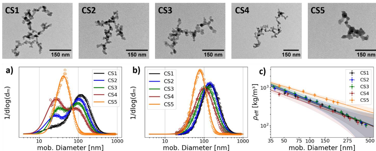
365 Figure 2 Top panel shows pictures illustrating the morphology of the five CS as obtained from TEM-imaging for samples collected 20 to 45 minutes after injection in CESAM. Bottom panel: number ( dN/d\log D_m ) size distribution measured (open circles) and fit-extrapolated log-normal size distribution (lines) of generated CS just after completion of the injection in CESAM (a) and 60 minutes later (b). Size data are normalized by the total number for each distribution. (c) Effective density ( \rho_{\text{eff}} ) as a function of mobility diameter ( D_m ) for the five CS as measured between a few minutes and 30 minutes after injection. The power-law fit (Eq. 5) is also plotted with its fitting uncertainty (shaded area).
