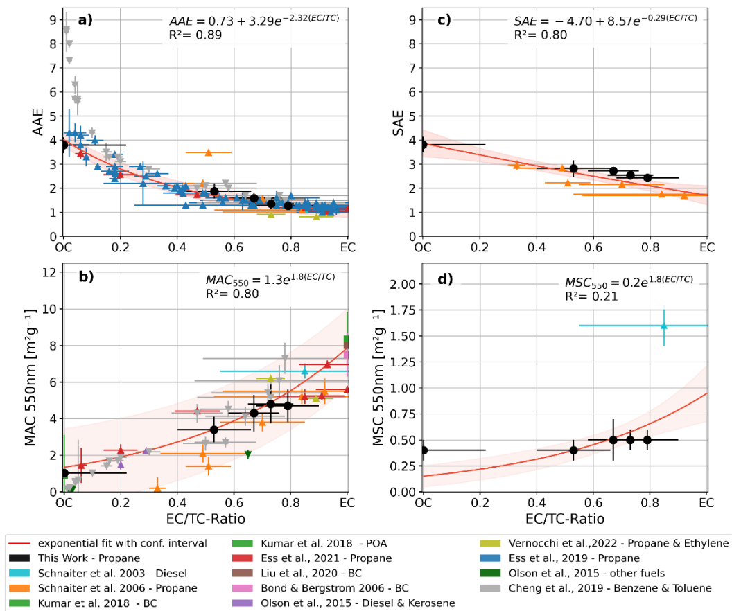
Figure 6 Compositional dependent absorption mass absorption and scattering cross sections (MAC, MSC) and their spectral variability represented by the absorption and scattering Ångström exponents (AAE, SAE). The MAC data obtained in the present study at 550 nm (black points) are combined with observations from past literature studies and put in relation to the EC/TC soot content. Data are fitted with the equation: y = a + b * e^{(c * EC/TC)} . Due to their fuel type, the soot produced by Cheng et al. (2019) (grey) and the other fuels from Olson et al. (2015), as well as values for pure BC and primary organic aerosols (POA) (Bond and Bergstrom, 2006; Kumar et al., 2018; Liu et al., 2020b), are not considered in the fits. In order to account for error bars in the fit an arbitrary minimal error of 10^{-3} was applied for EC/TC-ratios when these were not provided in their respective source studies. Any other uncertainty in the retrieved values was propagated according to the used calculation. The resulting equations for the absorbing properties are provided in the text and together with fits for the scattering in the supplements in Table S4.
