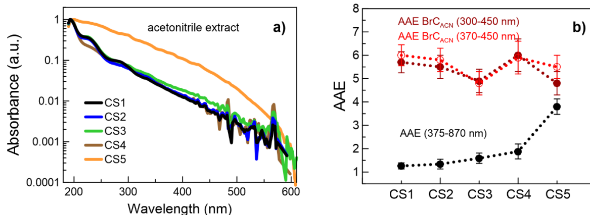
455 Figure 5 (a) Wavelength-dependent absorbance for acetonitrile soluble CS1-CS5 soot fraction. Absorbance data are normalised at the peak. (b) Comparison of the AAE obtained in the 300-450 nm and 370-450 nm ranges for the acetonitrile extracts and the AAE obtained for the soot aerosol within the 375-870 nm range.
