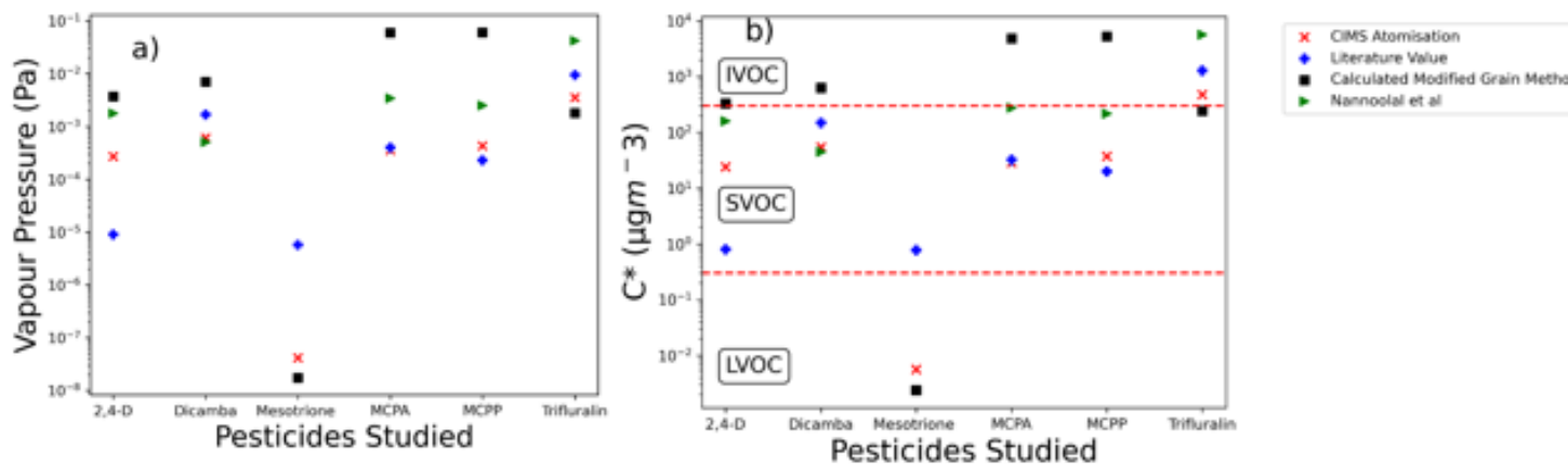
385 Figure 8 Measurement derived vapour pressure and C^* values of pesticides determined from T_{\max} data using the calibrations reported in section 3 and compared with accepted literature values from (Lewis et al., 2016), the Nannoolal et al method and the Modified Grain Method. . The red dotted lines represent the boundaries between the indicative volatility basis (VBS) categories defined by (Donahue et al., 2012b). The values come from the average of 3 runs shown in figure 7. The error bars are shown on the figure however are not visible due to the high repeatability.
