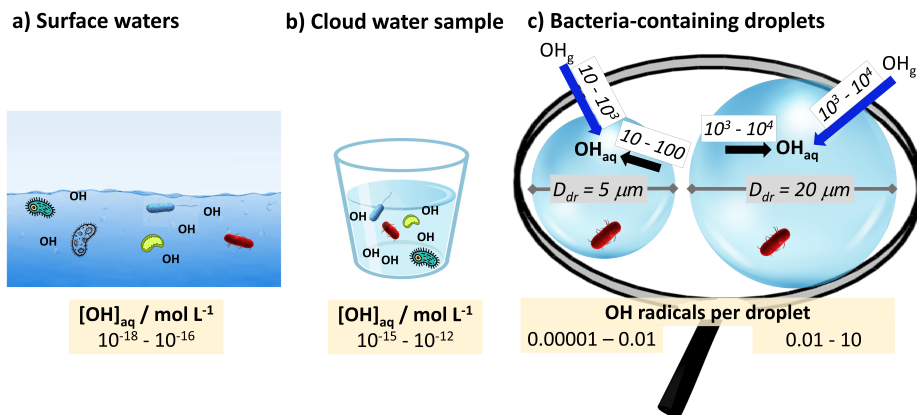
Figure 5. Concentrations of the OH radical in a) sea water (Mopper and Zhou, 1990); b) cloud water (Arakaki et al., 2013); c) individual cloud droplets ( D_{dr} = 5 \mu\text{m} , 20 \mu\text{m} ). The blue arrows in panel c denote the uptake rates of OH radicals per second, the black arrows denote their production rate inside a droplet (cf Figure S6c for individual reactions).
