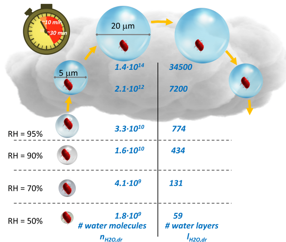
Figure 3. Number of water molecules ( n_{H_2O,dr} ) and water layers ( l_{H_2O,dr} ) under subsaturated conditions ( RH < 100\% ) and for cloud droplets with diameters of 5\ \mu m and 20\ \mu m (Section S2.1, supplemental information). The schematic suggests that under a wide range of atmospheric RH conditions, bacteria cells are surrounded by at least \sim 60 water layers which corresponds to about 20 mass% of the water in a bacteria cell ( m_{cell,H_2O} \sim 1.3 \cdot 10^{10} molecules water per cell). Since typical lifetimes of cloud droplets are on the order of 10 - 30 minutes, the largest water volumes may only represent very short-lived 'oases' (Section S2.2, supplemental information).
