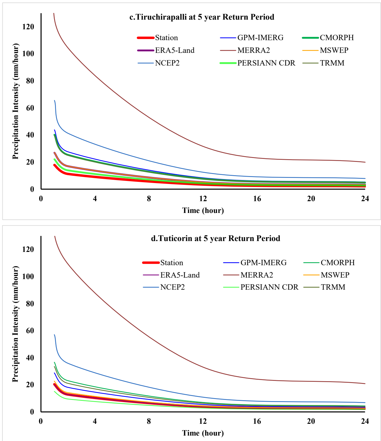
Figure 2. Intensity Duration Frequency (IDF) curves based on daily extreme (maximum) precipitation values for the study regions at 5 years return period
