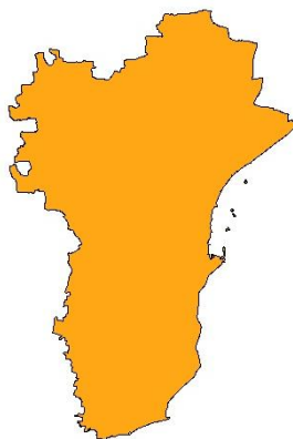
c. Tuticorin- GPM-IMERG
