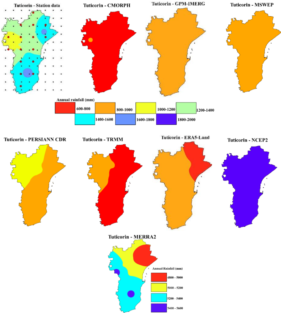
Figure 8. Mean annual precipitation for the Station-data and different precipitation products at Tuticorin. In the station data spatial map, red dots represent the station data, and black stars denote the linearly interpolated grids.
