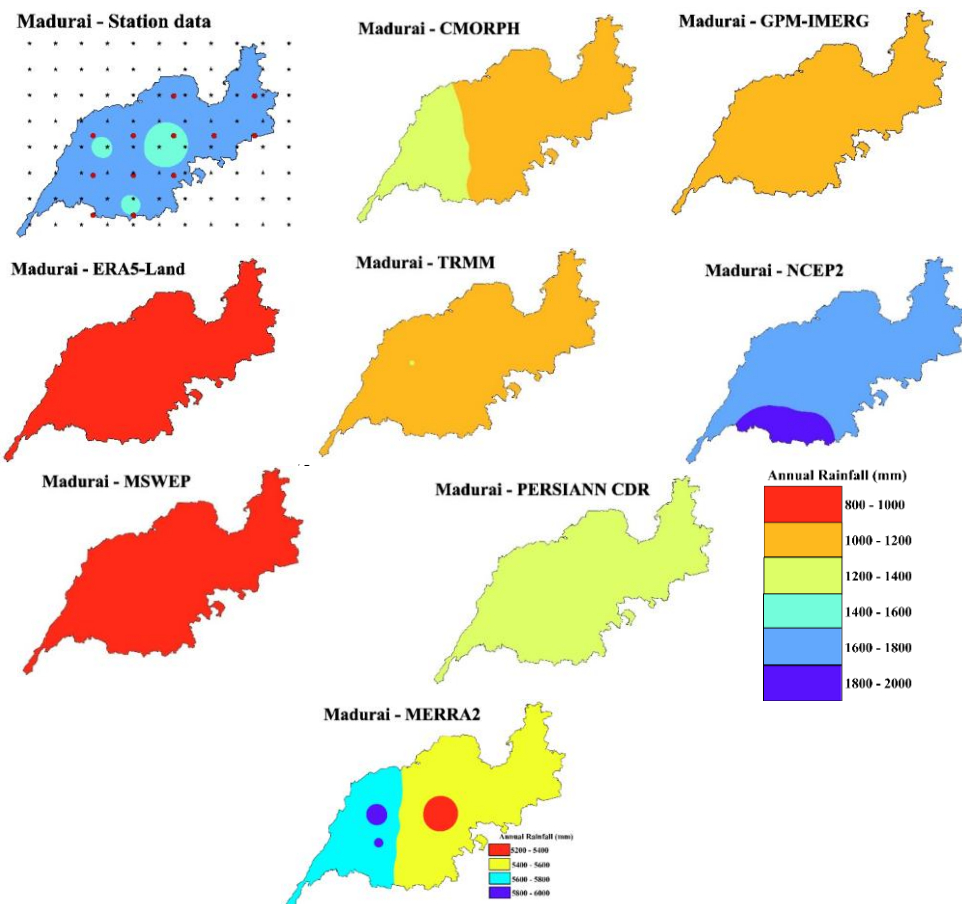
Figure 6. Mean annual precipitation for the Station data and different precipitation products at Madurai. In the station data spatial map, red dots represent the station data, and black stars denote the linearly interpolated grids.
