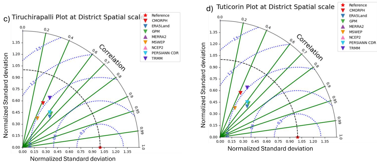
Figure S4 Taylor diagram depicting the agreement between station data and precipitation products at a yearly district scale
