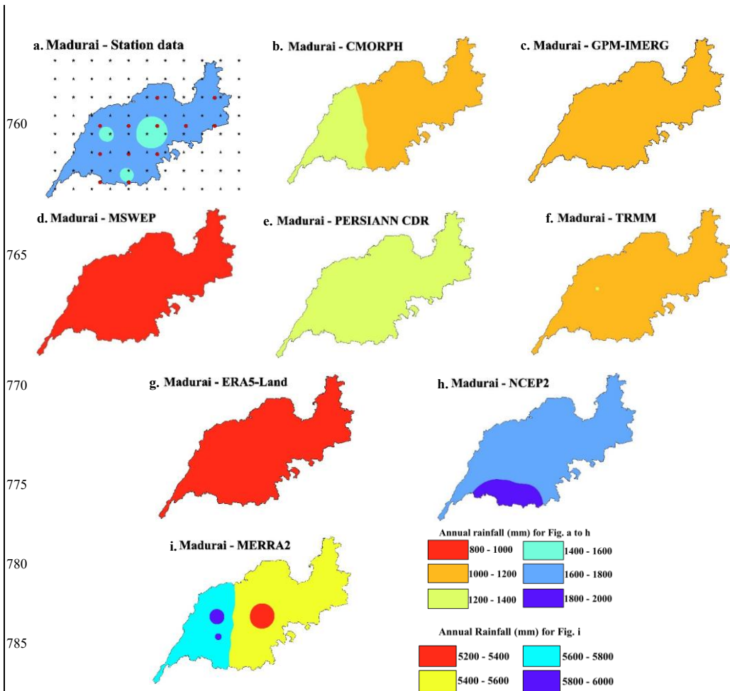
Figure 6. Mean annual precipitation for the Station data and different precipitation products at Madurai. In the station data spatial map, the distribution of ground station points and their respective linearly interpolated grids are plotted to understand the precipitation variation across the grids. The red circular dots represent the locations of ground stations from which precipitation data was collected for the period 2003–2014. The black stars indicate the linearly interpolated 0.1° grids. For the evaluation, only grids surrounded by at least one rain gauge were considered.
