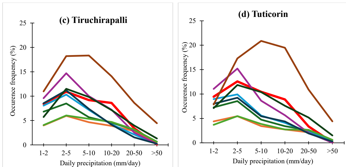
Figure S3 Occurrence frequency of precipitation (1-> 50 mm) for (a) Coimbatore, (b) Madurai, (c) Tiruchirapalli and (d) Tuticorin
