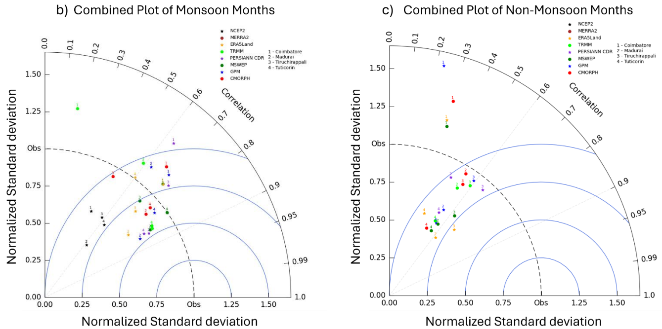
Figure S5 Combined Taylor diagram depicting the agreement between station data and precipitation products at a) yearly grid scale b) monsoon months c) non-monsoon months
