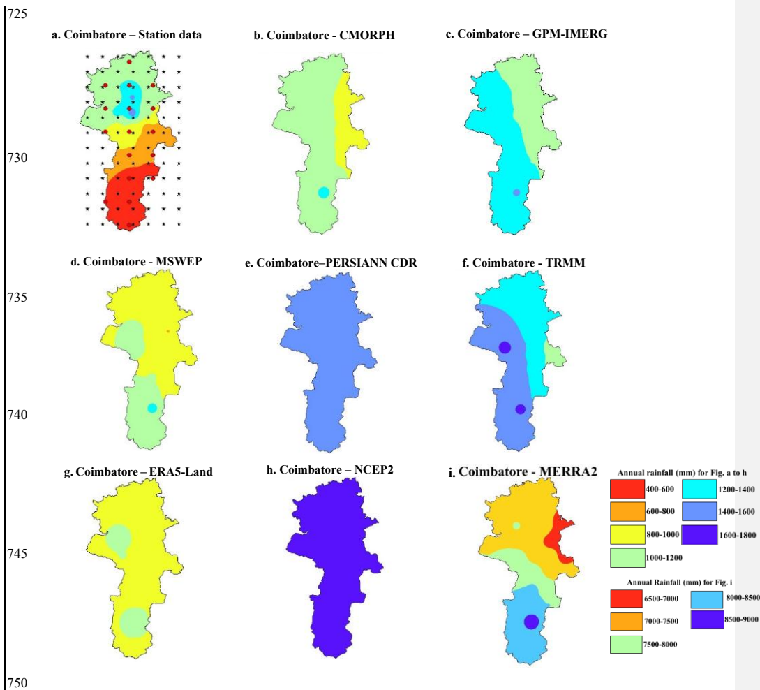
Figure 5. Mean annual precipitation for the Station data and different precipitation products at Coimbatore. In the station data spatial map, the distribution of ground station points and their respective linearly interpolated grids are plotted to understand the precipitation variation across the grids. The red circular dots represent the locations of ground stations from which precipitation data was collected for the period 2003–2014. The black stars indicate the linearly interpolated 0.1^\circ grids. For the evaluation, only grids surrounded by at least one rain gauge were considered.
