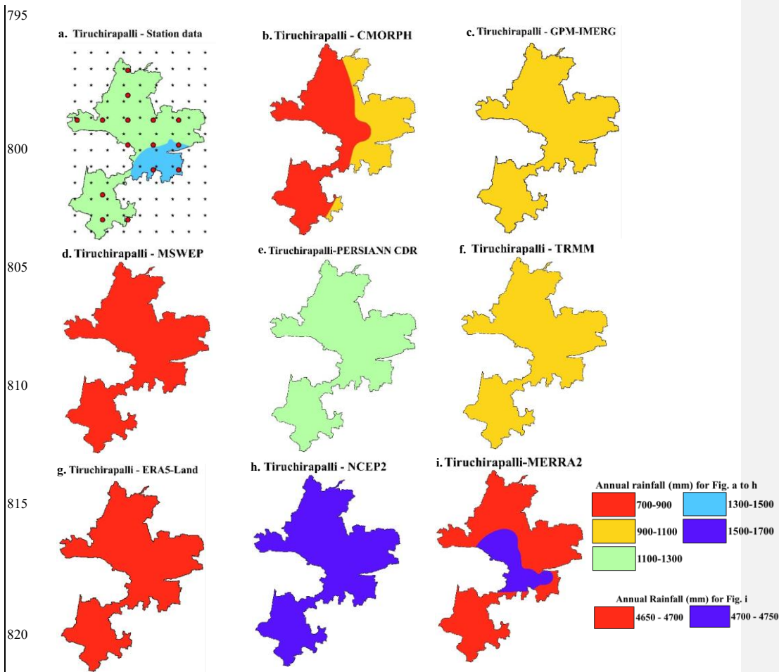
Figure 7. Mean annual precipitation for the Station data and different precipitation products at Tiruchirappalli. In the station data spatial map, the distribution of ground station points and their respective linearly interpolated grids are plotted to understand the precipitation variation across the grids. The red circular dots represent the locations of ground stations from which precipitation data was collected for the period 2003–2014. The black stars indicate the linearly interpolated 0.1^\circ grids. For the evaluation, only grids surrounded by at least one rain gauge were considered.
