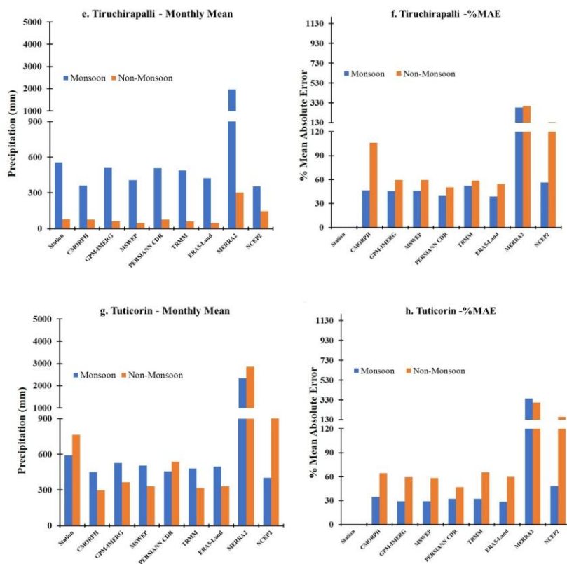
Figure 3. Monthly Mean and %MAE of different precipitation products with respect to Station data in Coimbatore (a,b), Madurai (c,d), Tiruchirappalli (e,f) and Tuticorin (g,h)
