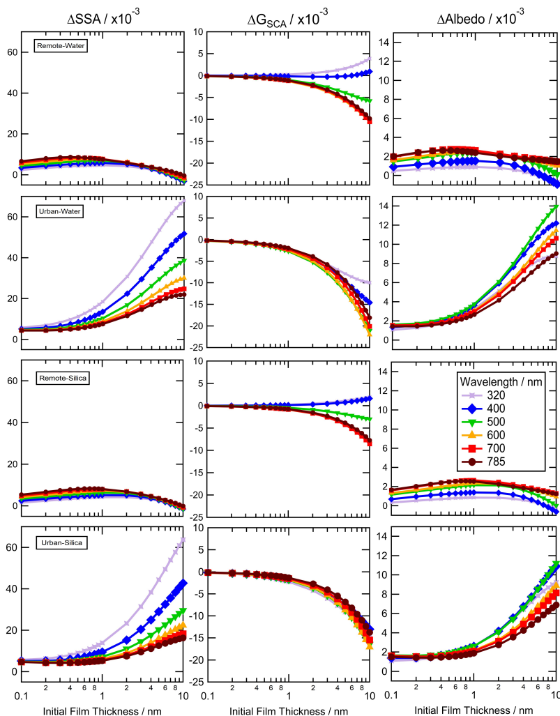
Figure 9. Change in aerosol single scattering albedo, \Delta SSA , asymmetry parameter, \Delta g_{sca} , and top of atmosphere albedo, \Delta Albedo , (80 km altitude, 60^\circ Solar zenith angle) calculated using a combination of Mie and 1-D radiative transfer modelling for the impact of the oxidation (represented by a halving of film thickness) of organic coated spherical silica and aqueous aerosol from urban and remote environments for wavelengths of light between 320–785 nm. Core and film materials were given complex refractive indexes representative of the material/environment. The single scattering albedo and asymmetrical light scattering of these four types of aerosol were calculated for aerosol with core sizes between 10–1000 nm with initial film thicknesses 0.1–10 nm, and normalised by the size distribution of aerosol from their respective environments. The single scattering albedo and asymmetry parameter were calculated for aerosol before and after oxidation. Radiative transfer models were produced for each aerosol disturbance, for each film thickness before and after oxidation. Values of single scattering albedo and asymmetry parameter were applied to a 3 km thick layer of aerosol at the planetary boundary layer, and top of atmosphere albedo was determined for a given model using aerosol with a given film thickness. \Delta SSA , \Delta g_{sca} and \Delta Albedo are the difference between the post-oxidation models from the pre-oxidation models.
