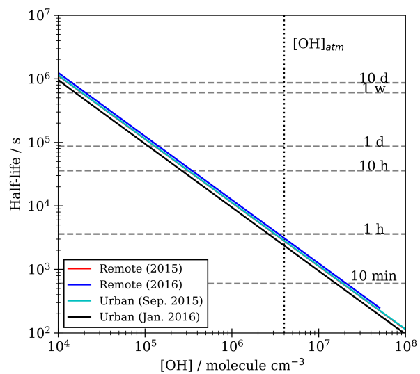
Figure 8. The half life of the film owing to chemicals oxidation by OH radical for different OH radical mixing ratios. A typical hydroxyl radical mixing ratio [OH]_{atm} is shown as a vertical dotted line.
