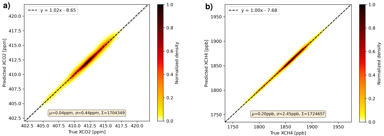
Figure 6. Comparison of postprocessed predicted XCO2 (a) and XCH4 (b) with corresponding true values for noise-free 2020 subset input data. \Delta represents the average prediction error (prediction minus true), \sigma the standard deviation of the prediction error, and \Sigma the total number of soundings. The figure also contains the results of a linear regression.
