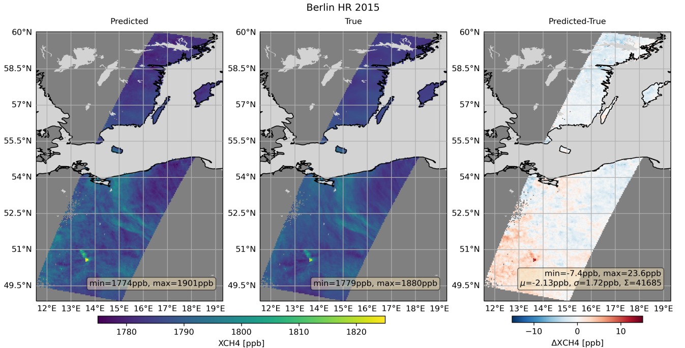
Figure 12. Postprocessed predicted XCH4 (left) and corresponding true values (middle) as well as their difference (right) for noise-free Berlin HR input data. \mu represents the average prediction error (prediction minus true), \sigma the standard deviation of the prediction error, and \Sigma the total number of soundings.
