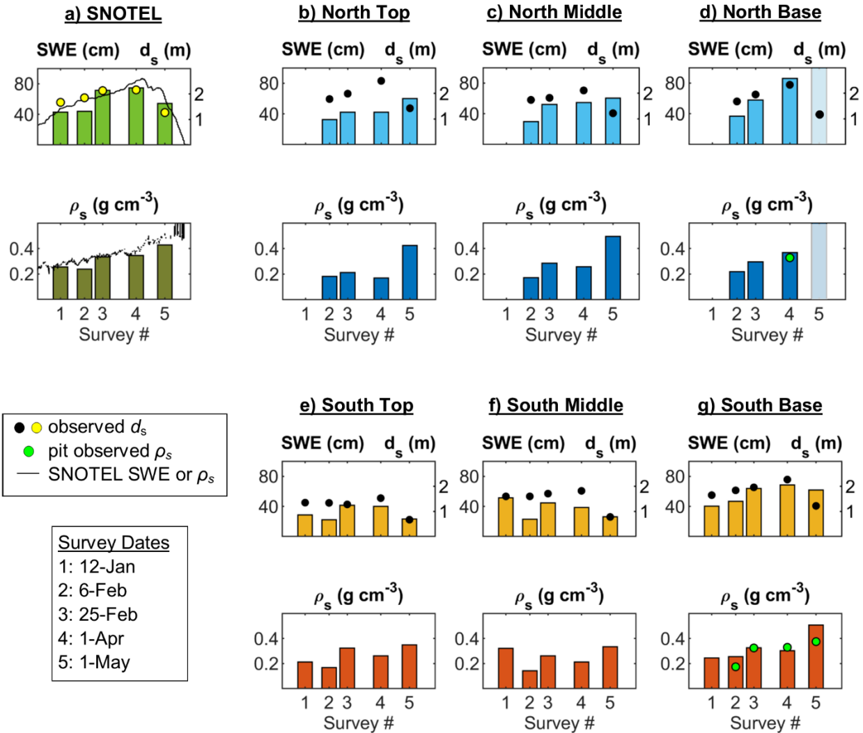
255 Figure 4: Results from the transect observations including calculated SWE, observed d_s , and GPR derived \rho_s for: a) Flat Terrain around the SNOTEL station, b) North Top, c) North Middle, d) North Base, e) South Top, f) South Middle, and g) South Base locations. Pit measured average densities are shown when collected, and SNOTEL station data are displayed for additional comparisons of SWE and \rho_s . Note that the GPR results that gave unrealistic values due to the presence of liquid water is slightly greyed in panel d.
