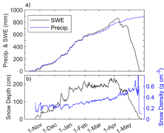
200 Figure 3: SNOTEL data for the 2023 water year showing a) observed SWE and cumulative precipitation, and b) observed snow depth and calculated snow density.
