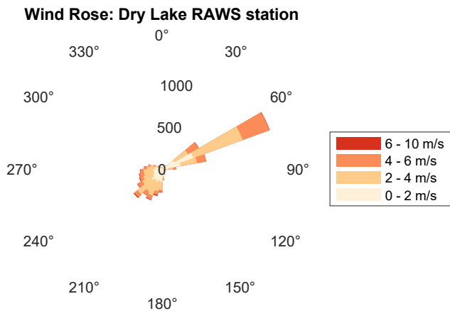
Figure A1. Wind rose for the Dry Lake RAWS site.
