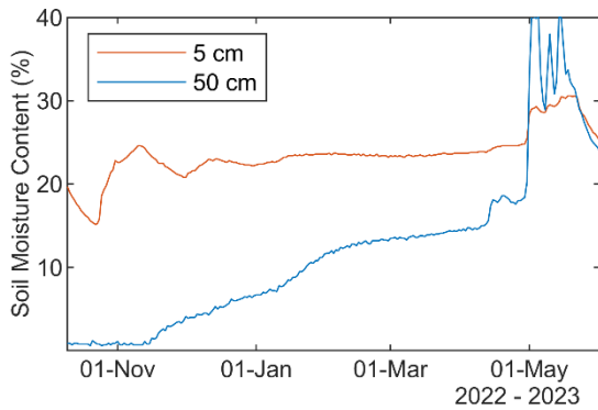
260 Figure 5: Soil moisture data from the SNOTEL site at depths of 5 cm and 50 cm.
