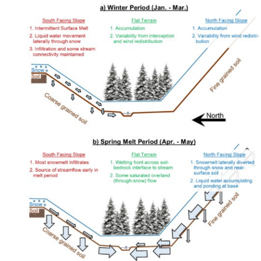
Figure 8: Perceptual model of interpretation of processes during a) the winter period (January through March) and b) spring melt period (April through May). Panel (b) is modified from Webb et al. (2018a).
