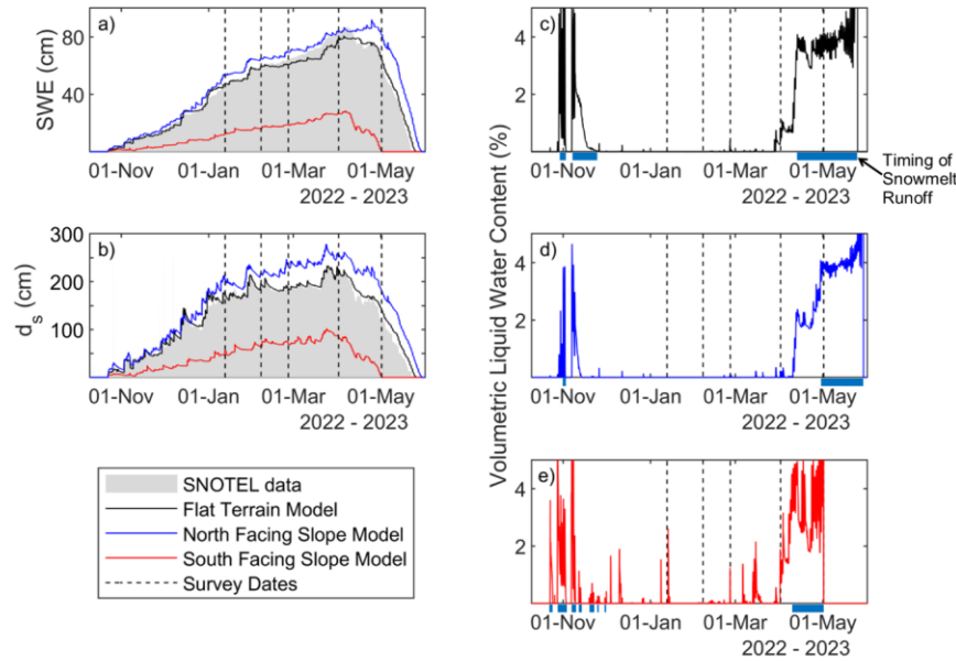
Figure 7: Results from the SNOWPACK simulations including a) SWE, b) d_s , and c) – e) volumetric liquid water content. Panels c) – e) also show when simulated snowmelt runoff from the snowpack is occurring as blue bars. Results show comparison to SNOTEL data as well as timing with survey dates.
