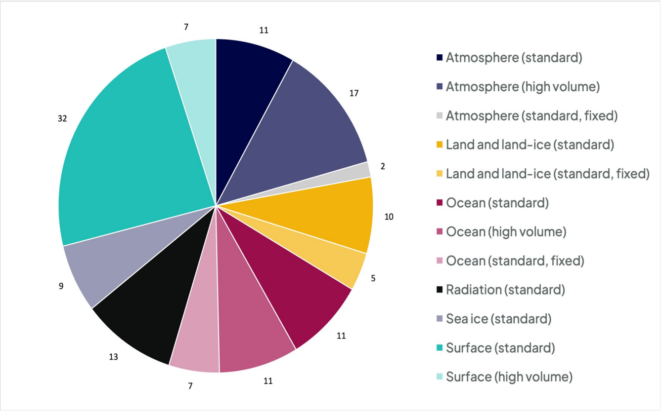
361 Figure 5: ESM baseline climate variable categories. Distribution of ESM-BCVs across a range of categories (using the data listed 362 in Table A7, Appendix C). A variable is considered as “high-volume” (dark shading) if 10 thousand years of simulation generates 363 more than 1,500 GB of data from a 1-degree resolution model with 60 atmospheric levels and 500 oceanic levels archived 364 (assuming single precision data storage without compression).
