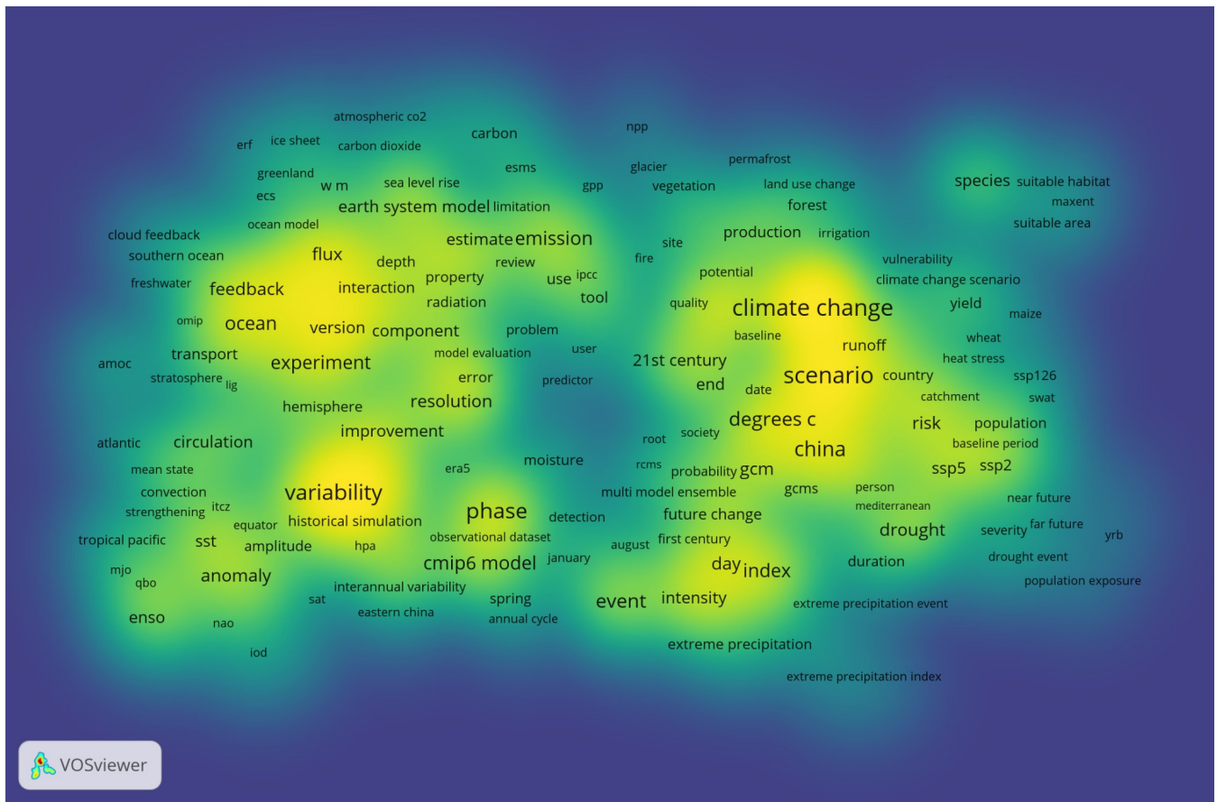
Figure 3: Word cloud of CMIP6 science. Word cloud generated by analysis of titles and abstracts of 5152 Web of Science articles. Words are grouped according to closeness defined by the frequency with which they appear in the same papers. Yellow indicates clustering of more commonly used words. Generated by VOSViewer.
