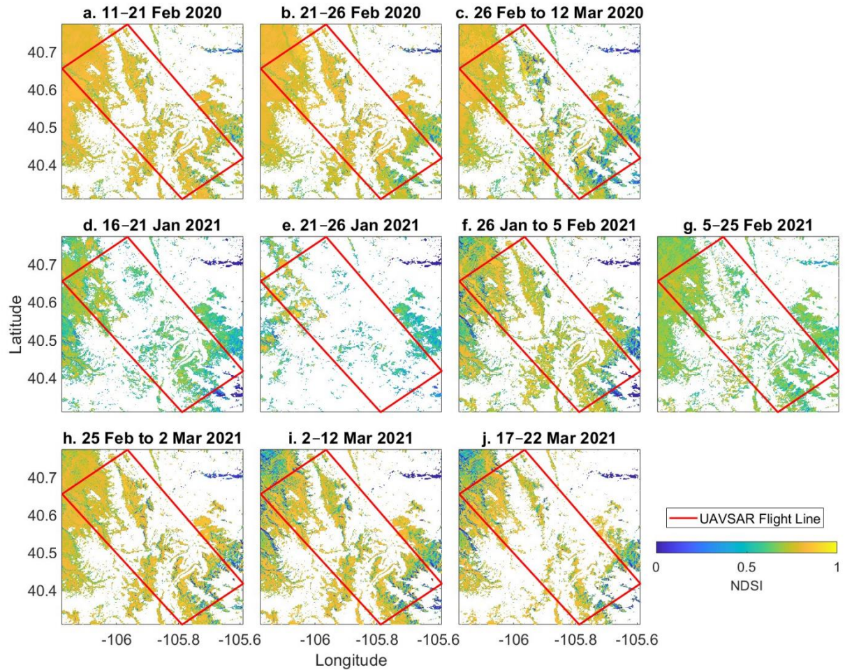
Figure S1: (a) NDSI (Equation A2) maps for each UAVSAR flight interval calculated from composited Sentinel-2 Level 2A imagery. Clouds and forests were removed from this analysis. Snow-free pixels were identified as \text{NDSI} < 0.20 .
