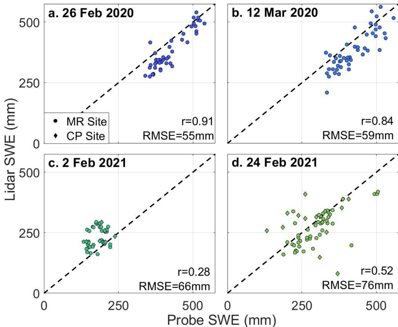
Figure S3: Comparisons between TLS SWE retrievals and SWE converted from probed depths for each lidar survey date. Probed SWE points represent the average of the one to two probed points within a single TLS pixel. The TLS survey conducted on 10 February 2021 was adjusted to 2 February 2021 by using SWE measured on the interval board on 10 February 2021. Overall Pearson's correlation coefficient = 0.83 and RMSE = 66mm. Points are colored by date, following Figure 8a–c.
