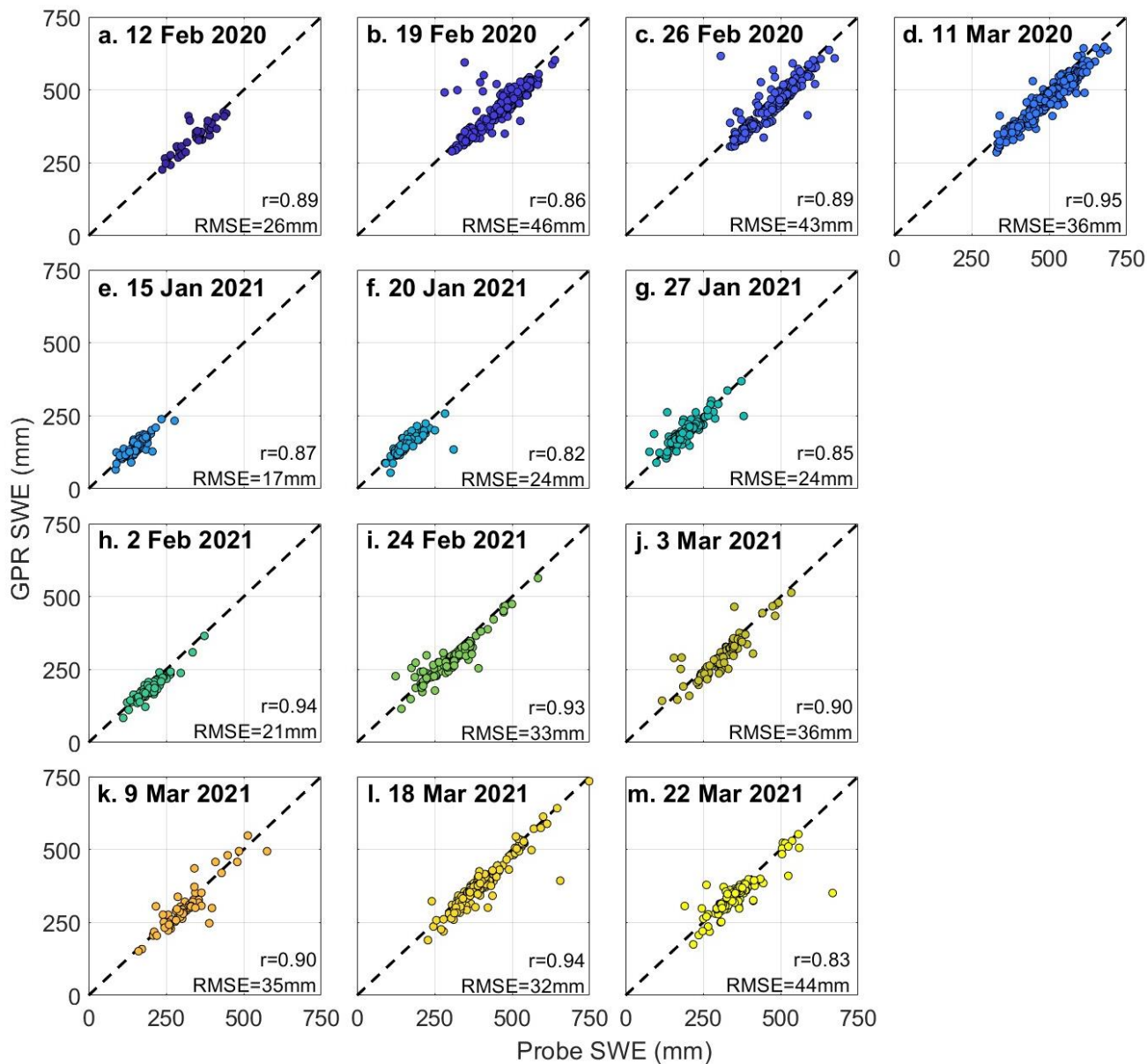
60 Figure S2: Comparison between GPR SWE retrievals and SWE converted from probed depths for each survey date. Median GPR SWE was calculated within a 1.5 m radius for each probed point. The number of GPR points used for estimating the median GPR SWE for comparison with probed SWE varied, but in most cases, exceeded 10 points per probe. Points are colored by date, following Figure 8a-c. In 2020, ~200 probed points were collected per survey date, whereas ~120 were collected per survey date in 2021. Overall Pearson's correlation coefficient = 0.97 and RMSE = 35 mm.
