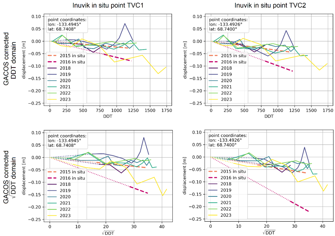
Figure 1: Comparison of displacement time series for two sample points with in situ subsidence measurements for the years 2015 and 2016 near the Trail Valley Creek (TVC) research station (Inuvik region). The top figures display GACOS corrected results in the DDT domain while the lower figures show GACOS corrected results in the \sqrt{DDT} domain.
