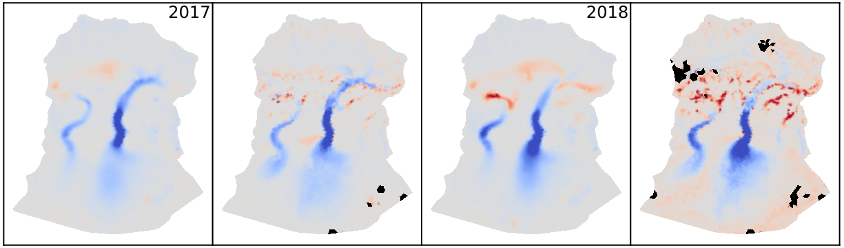
Fig. S1: Modelled (left) and observed (Right) ice speed anomalies for all years with a velocity observation. The color scale saturates at -200 \text{ m a}^{-1} and 200 \text{ m a}^{-1} .
