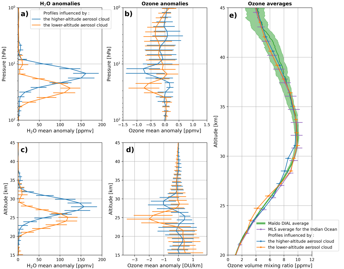
Figure 6. Mean anomalies and \pm 1\sigma standard deviation (horizontal bars) in (a-c) water vapor and (b-d) ozone from v4 MLS profiles that met the selection criterion. Panels (a-b) presents present measurements from raw profiles in volume mixing ratio over a pressure range, while panels (c-d) shows show the same data over an altitude range, with ozone expressed in DU/km. Panel (e) displays the January mean lidar ozone profile with its \pm 2\sigma standard deviation, the MLS average ozone profile for the Indian Ocean with its \pm 1\sigma standard deviation, and the average v4 MLS ozone profiles influenced by one-of-the aerosol-Hunga clouds with the corresponding \pm 1\sigma standard deviation. Profiles influenced by the higher-altitude and lower-altitude sulfate-aerosol clouds are displayed in blue and orange, respectively.
