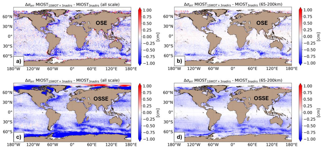
Figure A1: Gain/loss of the mapping error standard deviation of SLA when integrating SWOT into a 3 altimeters constellation for a) all spatial scale in OSE, b) scale < 200km in OSE, c) all spatial scale in OSSE, and d) scale < 200km in OSSE. Blue colour means a reduction of error standard deviation when SWOT is included in the mapping.
