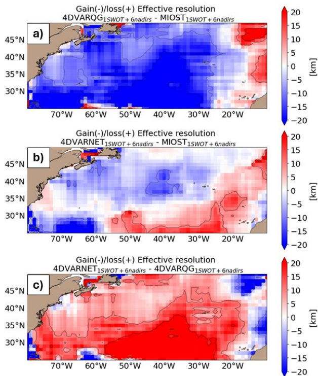
495 Figure B4: Gain/loss of effective resolution (in km) between a) the 4DVARQG and MIOST mapping methods (Blue means finer resolution with 4DvarQG), b) the 4DVARNET and MIOST mapping methods (Blue means finer resolution with 4DvarNET) and c) the 4DvarNET and 4DvarQG mapping method (Blue means finer resolution with 4DvarNET)
