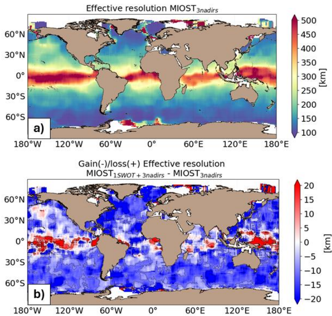
290 Figure 7: Maps of effective spatial resolution (in km) for (a) the 3 nadirs experiment and (b) gain/loss of effective resolution (in km) between the 1 SWOT + 3 nadirs experiment and the 3 nadirs experiment. Blue means finer resolution when SWOT is included in the mapping.
