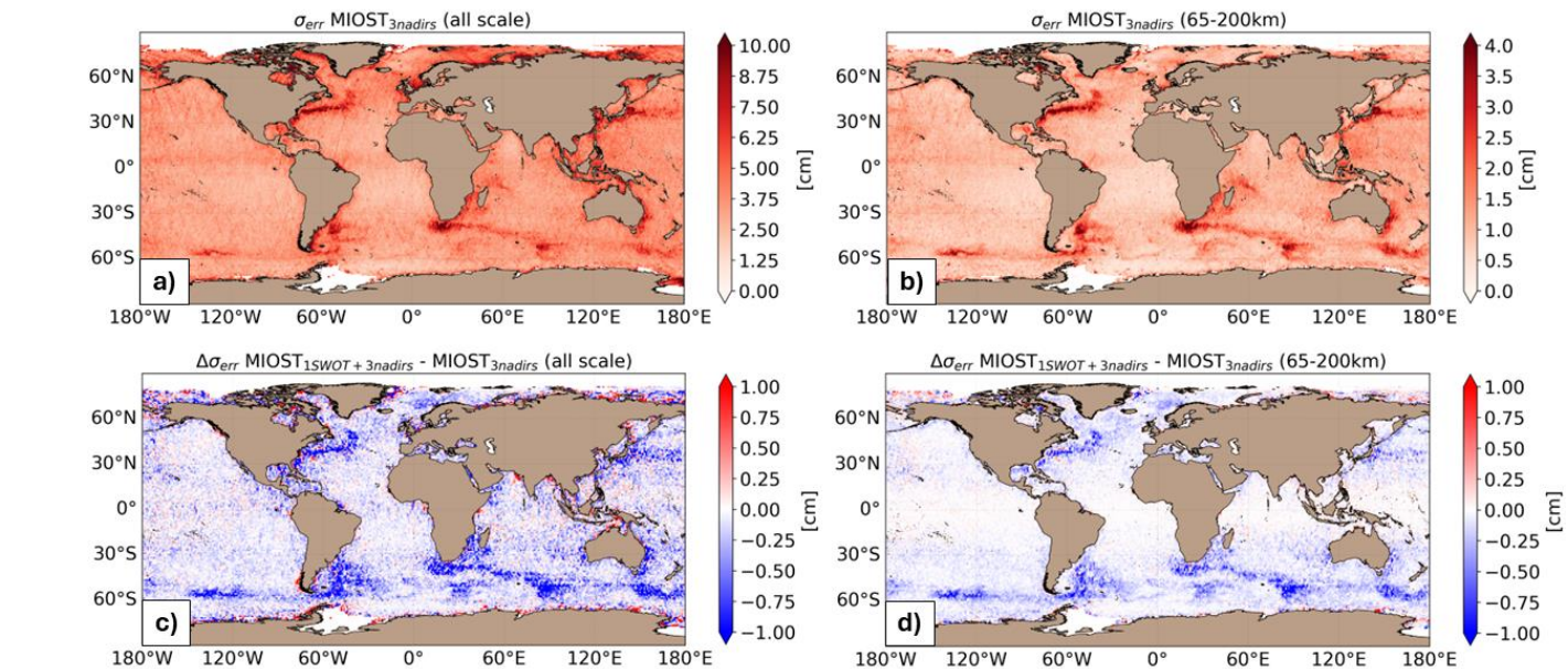
Figure 6: Standard deviation of the difference SSH_{map} - SSH_{alongtrack} computed for the 3 nadirs experiment and in considering a) all spatial scale and b) spatial scale between 65 km and 200 km. Gain/loss of the mapping error standard deviation of SLA in 3 nadirs + 1 SWOT experiment relatively to the 3 nadirs experiment mapping error standard deviation for c) all spatial scale and d) scale between 65 km and 200 km. Blue colour means a reduction of error when SWOT is included in the mapping.
