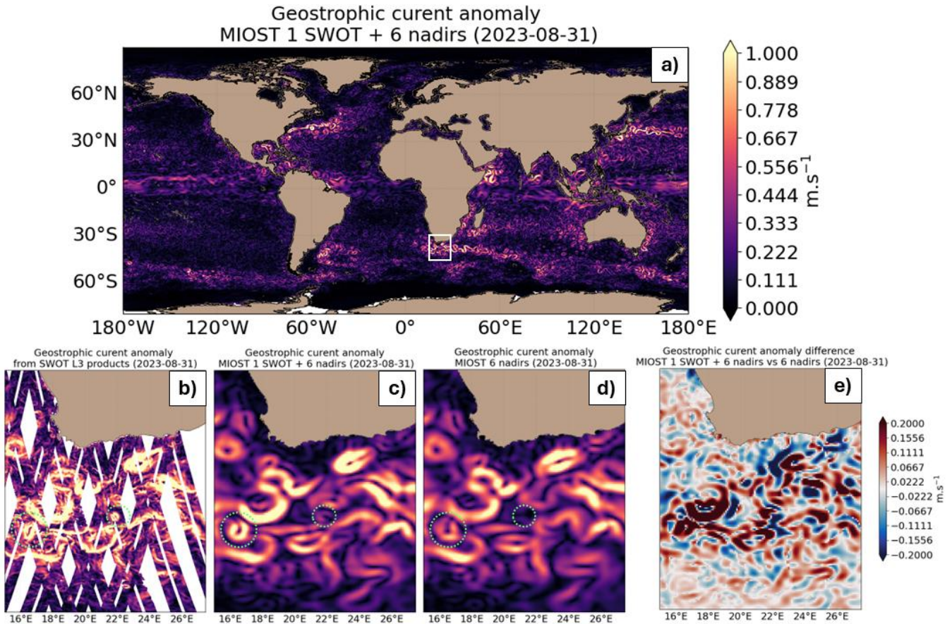
Figure 3: Example of geostrophic current reconstruction on 2023-08-31 with MIOST at a) global scale, b) view from Karin L3 products over the Agulhas region, c) from MIOST reconstruction integration 1SWOT and 6 nadirs, d) from MIOST reconstruction integration 6 nadirs and e) the difference in MIOST reconstructions between integration 1SWOT and 6 nadirs vs 6 nadirs only
