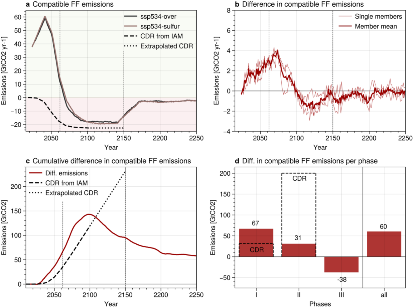
Figure 3: a) compatible fossil fuel emissions for SSP534-over (black) and SSP534-sulfur (taupe). Dashed line shows the amount of negative emissions implemented in the IAM ssp534-over scenario (Byers et al., 2022). b) SSP534-sulfur – SSP534-over. c) Shows values of b in a cumulative manner. d) shows values of b when summed over the single peak-shaving phases (I, II and III) and summed over the entire time frame (all). The stippled CDR-boxes indicate required CDR during the respective period. Stippled vertical lines indicate the overshoot phases I, II and III. Data for these plots are based on the ensemble mean of the three members except in b) where the single member differences are displayed in thin red lines.
