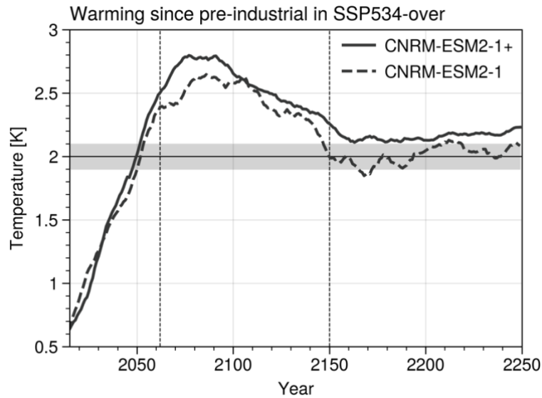
Figure 2: 10-year rolling mean warming in the overshoot scenario SSP534-over simulated by the model version used in this study (CNRM-ESM2-1+; solid) and the former model version (CNRM-ESM2-1; dashed). Lines represent the mean of a 3-member ensemble. The gray zone indicates the 0.1°C tolerance level around the 2°C temperature target. Stippled vertical lines indicate the overshoot phases I, II and III.
