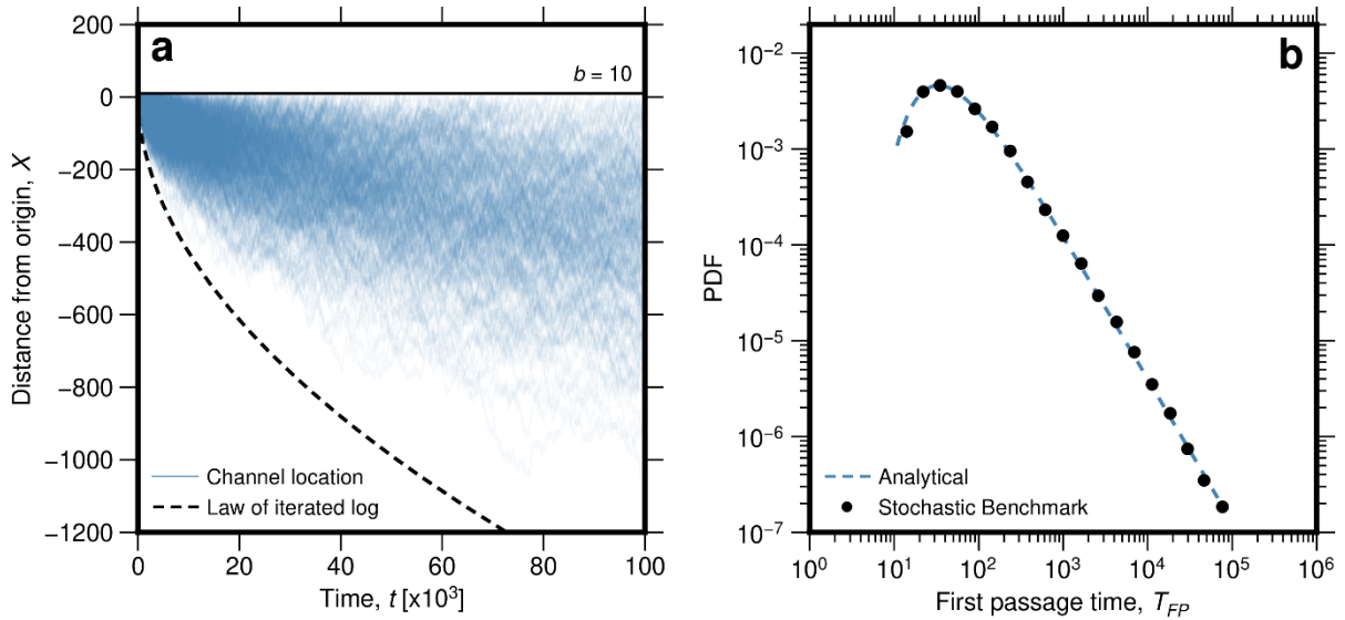
558 Fig. 5: The results for the first passage distribution. a) Paths of models to investigate time distribution to reach a point 559 a distance b from the origin (horizontal black line). The dashed line gives the expectation from the law of the iterated 560 logarithm (eq. 32). In comparison to Fig. 2a, substantially longer runs in time are shown here. b) First passage time 561 distribution of the Stochastic Benchmark (black dots show binned means) in comparison to the analytical solution 562 (dotted blue line, eq. 33).
