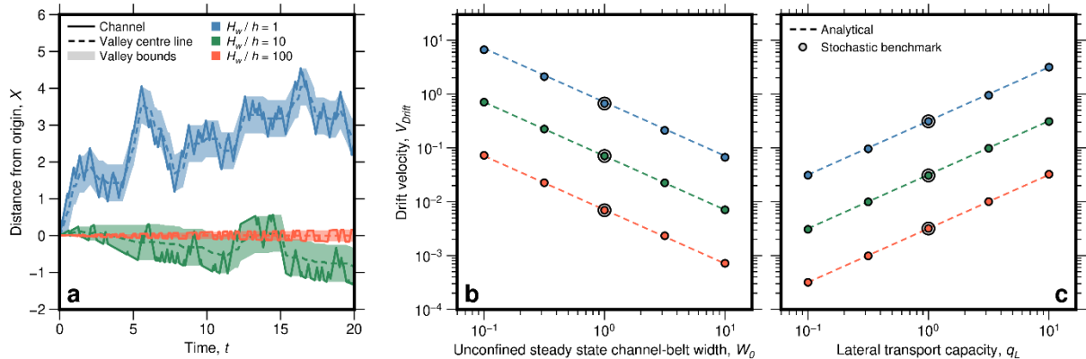
Fig. 3: Lateral drift speed of channel belts at constant steady state width for the drift-phase. For the calculation, channel-belt width was fixed to the steady state width, i.e., whenever the channel widened the channel belt on one side, the width was reduced by the same amount on the other side. a) Channel location as a function of time for different degrees of confinement (same colour code as in Fig. 2). Note that a) does not show the entire calculated trajectories; average drift velocities were measured after 10,000 steps. b) Average drift speed as a function of steady width from the Stochastic Benchmark are shown as circles. The analytical predictions (dotted lines) of eq. (29) fit the numerical results well. c) Average drift speed as a function of lateral transport capacity with the same symbology as in b). Larger circles in b) and c) show simulations plotted in a).
