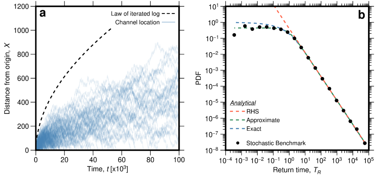
565 Fig. 6: The analytical results for the return time distribution, equivalent to the age distribution of sediments stored in 566 the channel belt and comparison to data. a) Paths of 10,000 models to investigate the time distribution for the return 567 to the origin. Once a model path reached the origin, later timesteps are not plotted. The dashed line gives the prediction 568 of the return time from the law of the iterated logarithm (eq. 32). In comparison to Fig. 2a, substantially longer runs 569 in time are shown here. b) Modelled return time distribution (black dots show binned means) compared to the exact 570 analytical solution (blue, eq. 34), the power law decay in the right-hand tail with an exponent of -3/2 (red, eq. 35). The 571 analytical approximation (green, eq. 36) is also shown.
