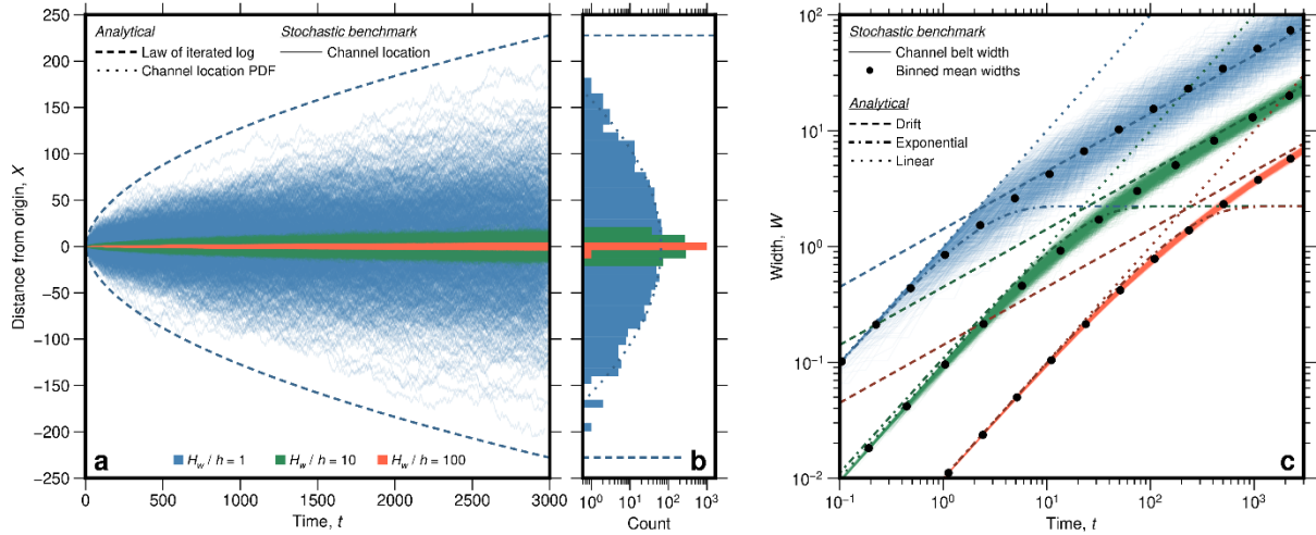
Fig. 2: Temporal evolution of channel-belt width in the Stochastic Benchmark and comparison between the Stochastic Benchmark and the analytical solutions. a) Modelled migration paths through time (coloured solid lines), bounded by the law of the iterated logarithm (dashed line, eq. 32), i.e., the area that the river almost surely does not crosses. Similar plots with longer runtimes can be found in Fig. 5a and Fig. 6a. The blue lines show the evolution of an unconfined river ( H_w/h = 1 ), the green lines show a moderately confined case ( H_w/h = 10 ), and the orange lines a highly confined case ( H_w/h = 100 ). b) Location density at t = 3000 . The dotted line gives the theoretically expected normal distribution for the unconfined case (blue), the dashed line marks the law of the iterated logarithm. c) Average width evolution with time, showing the analytical expressions for the linear (dotted lines, eq. 1), exponential (dash-dotted lines eq. 12) and drift phases (dashed lines eq. 25). Fine solid lines show the outputs from the numerical simulation and black circles show the mean widths of these simulations in bins spaced logarithmically in time. Standard errors of the means are smaller than the symbols.
