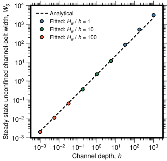
550 Fig. 4: Verifying the value of the constant c (see eq. 30) by comparing unconfined steady state channel-belt width 551 obtained from fits to the Stochastic Poisson Model (Fig. 1) to channel depth for varying simulations. We set channel 552 width W_C = 0 and k = 1 for these simulations. Then, the steady state channel-belt width and flow depth should be 553 proportional with a constant of proportionality equal to 1/c (eq. 4). The dashed line gives the theoretically expected 554 relationship with c = 2.2285 (eq. 30). The results show that the value of c is the same for unconfined and confined 555 channel belts.
