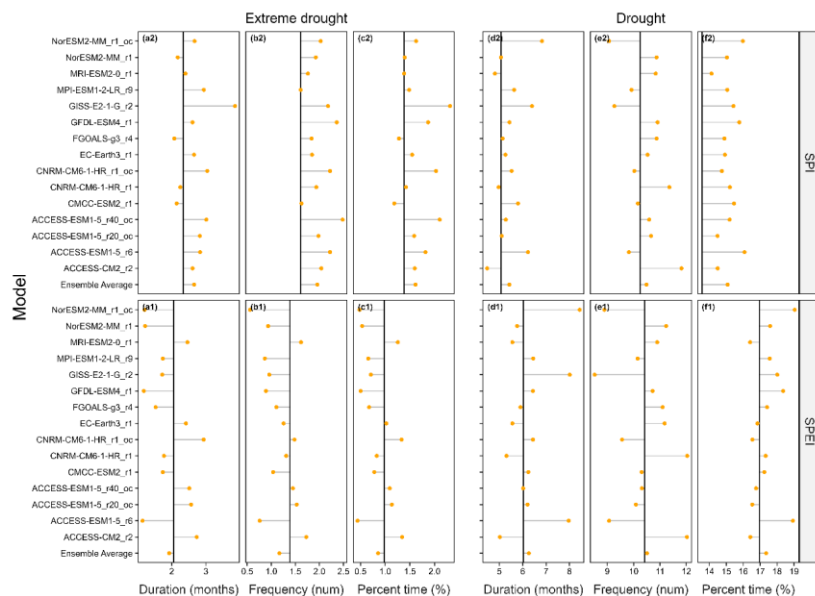
Figure 2: Comparison of the differences in calculated metrics of drought and extreme droughts between climate model simulations and observations for the historical calibration period over all of Australia (1981 to 2010). Drought metrics from observation data are presented as solid black lines, while points show metrics from climate model simulations.
