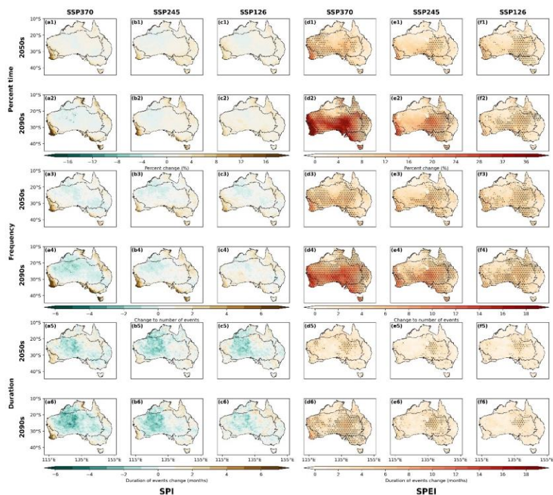
Figure 10: Maps showing changes to the percent time (rows 1 to 2), frequency (rows 3 to 4), and duration (rows 5 to 6) of extreme droughts according to SPI (columns a, b, and c) and SPEI (column d, e, and f) for the 2050s and 2090s relative to the reference period. Hatching shows where the signal-to-noise ratio > 1.0.
