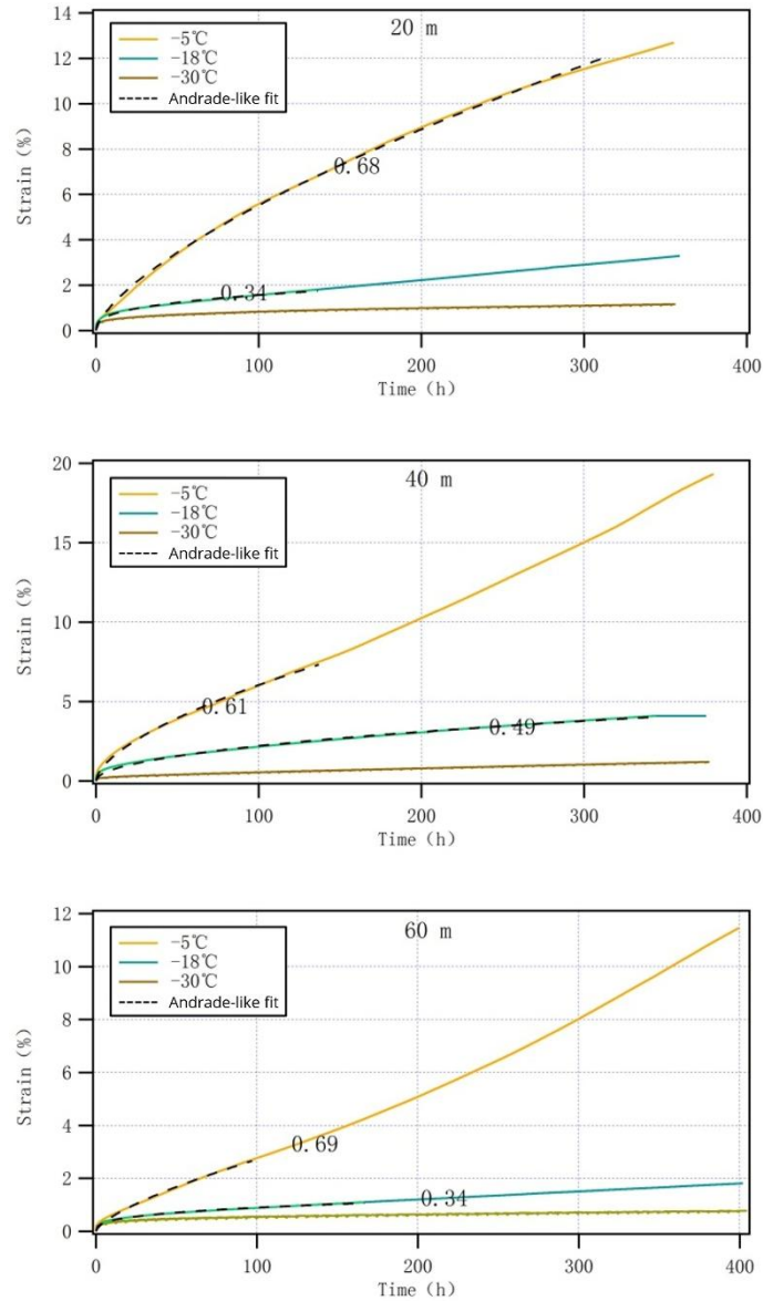
367 Figure 5: Strain vs. time for firm specimens at -5^{\circ}\text{C} (yellow lines), -18^{\circ}\text{C} (blue lines), and -30^{\circ}\text{C} 368 (brown lines), from depths of 20 m (applied stress 0.21 MPa), 40 m (0.32 MPa) and 60 m (0.43 369 MPa). The black dashed curves represent fits to a modified Andrade-like equation with the time 370 exponents indicated on the curves, if any. Note: The y-axis limits vary across the subfigures.
