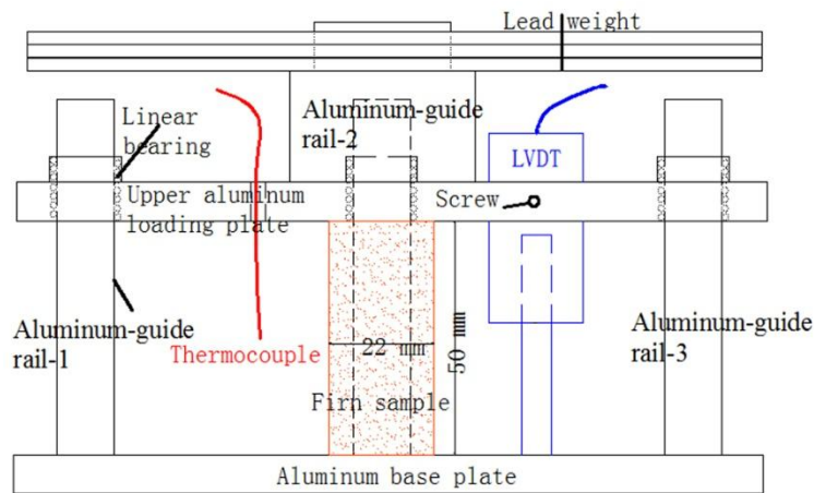
178 Figure 1: Schematic illustrating the home-built compressive creep jigs. More details can be found 179 in (Li & Baker, 2022a).
