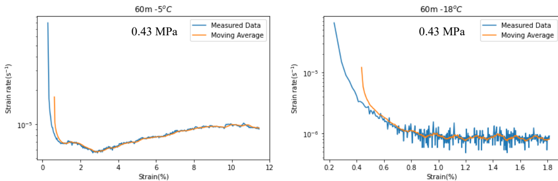
415 Figure 6: Log strain rate vs. strain from the firm specimens at temperatures of -5°C and -18°C 416 from depths of 20 m (applied stress 0.21 MPa), 40 m (0.32MPa) and 60 m (0.43MPa). Samples 417 from -30°C are not shown due to the very large noise. The blue lines represent discrete strain rates, 418 which are calculated by extracting the strain data hourly, while the orange lines represent a 419 moving average of 15 moving windows with respect to the strain.
