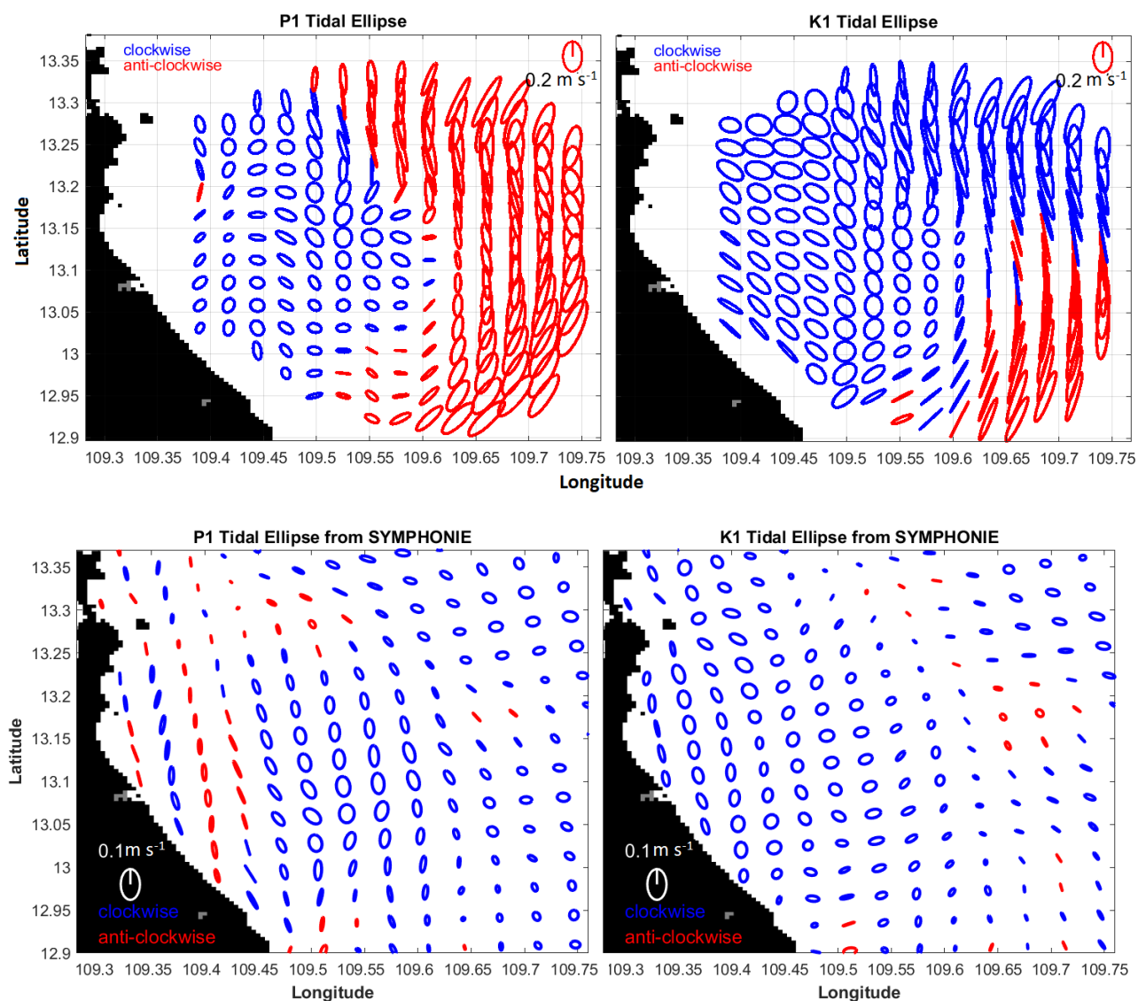
Figure 4: Tidal ellipse distribution for P1 constituent (left) and K1 constituent (right) from HFR (top row) and from VMSC_ref (bottom row)
