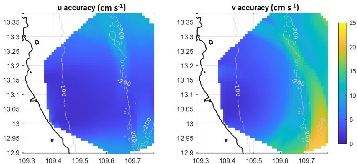
445 Figure A1: Mean accuracy map of u and v components of sea surface currents from HFR measurements for the entire period of measurements.
