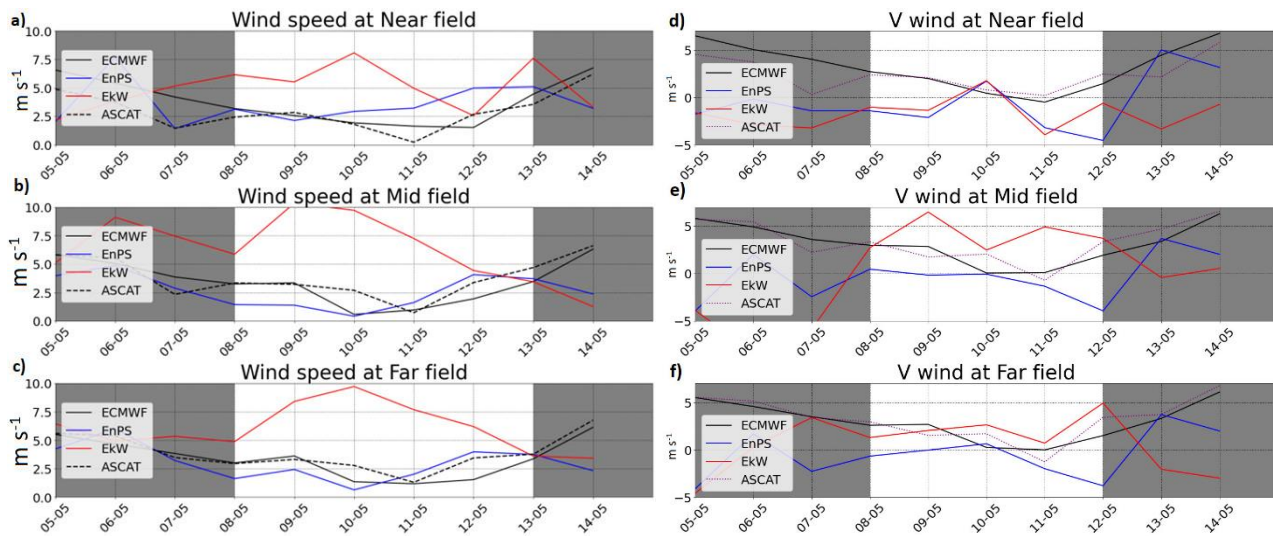
320 Figure 10: Columns: Wind speed time-series from different wind data (left column); Time series of V-component of wind from wind data (right column); Rows: three sub-domains: near field, mid field and far field
