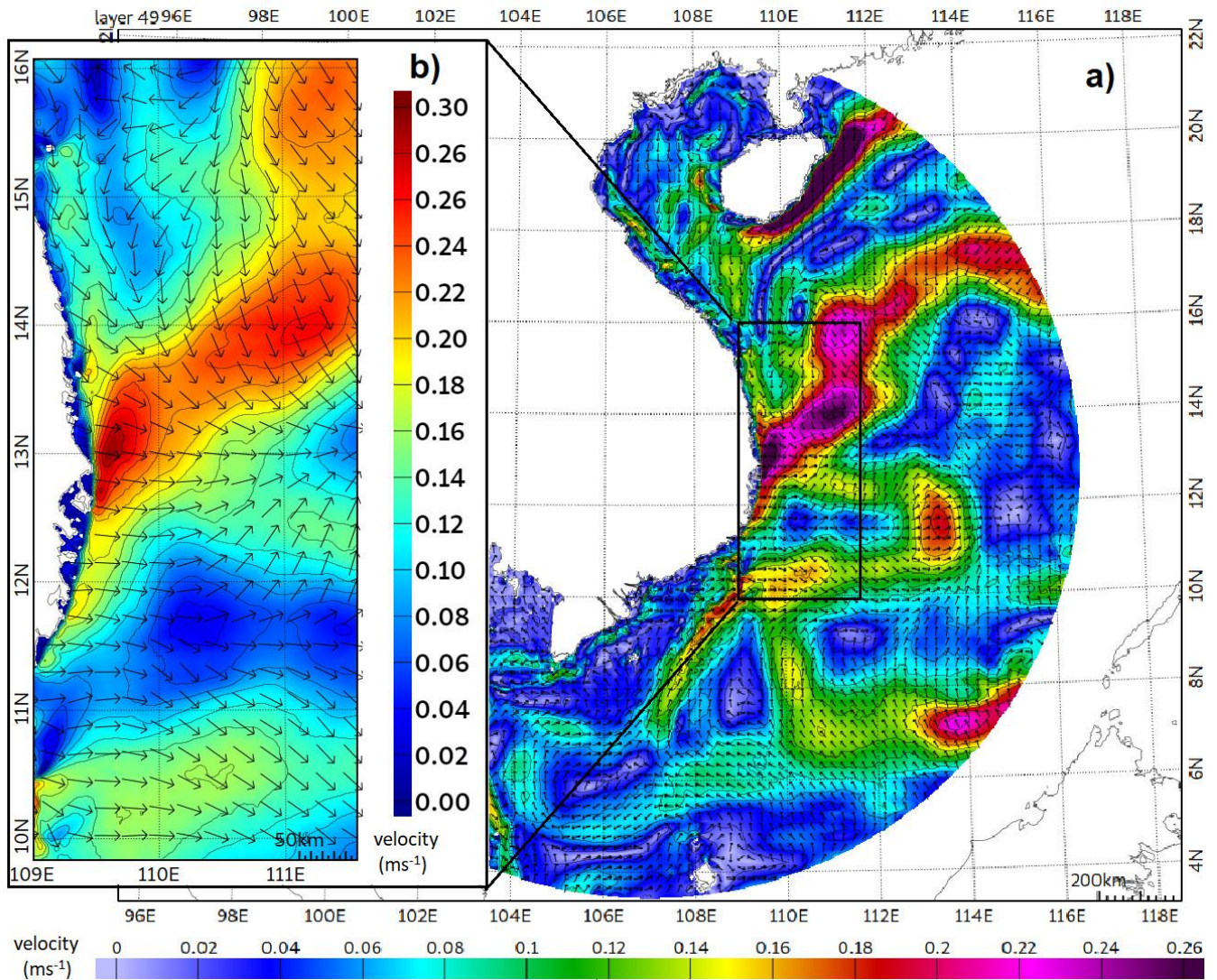
270 Figure 5: a) Surface circulation in the western SCS in April-May, from the EASTSEA run. The current velocity fields have been averaged for the 10-year period, 2009-2018. b) A zoom-in to the VMSC domain. The colour scale depicts the velocity of surface currents in \text{ms}^{-1} . A large upwelling and current separation already occur at latitudes 10-14°N during this time of the year (Tran et al., 2022)
