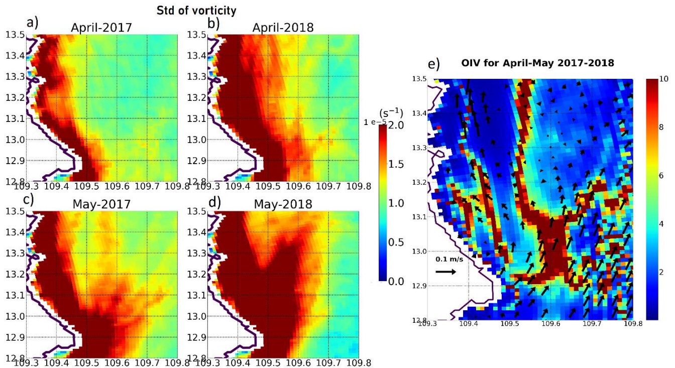
385 Figure 12 (a-d) Monthly mean standard deviation of SSC vorticity over ensembles; e) OIV index superimposed with multi-annual monthly average SSC vectors for April-May, 2017-2018
