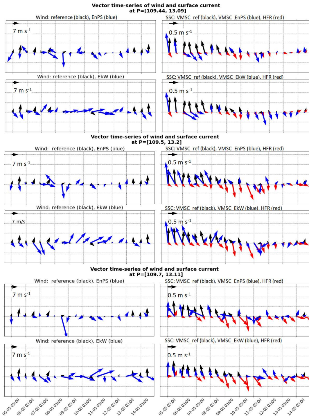
320 Figure 9: Vector time series of wind (reference, EnPS, EkW) and SSC (VMSC_ref, VMSC_EnPS, VMSC_EkW and HFR) of three points located at near-, mid- and far-field of the HFR domain.
