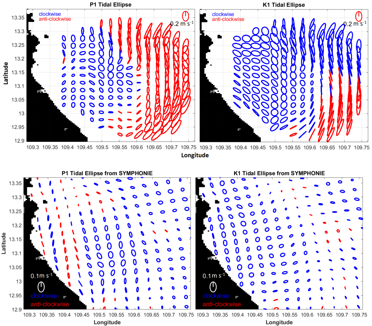
250 Figure 4: Tidal ellipse distribution for P1 constituent (left) and K1 constituent (right) from HFR (top row) and from VMSC_ref (bottom row)
