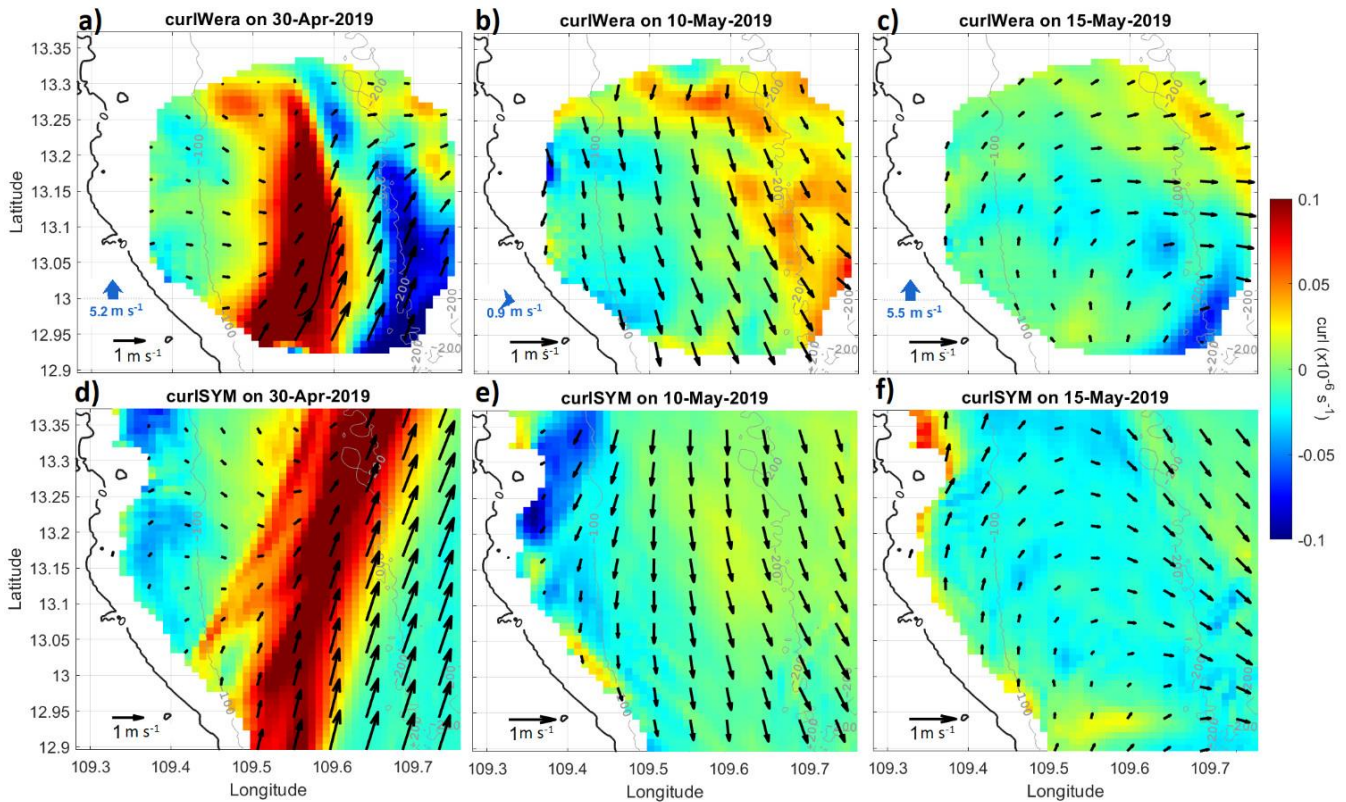
275 Figure 6: SSC vectors obtained from HFR (a-c) and SYMPHONIE (EASTSEA run) (d-e) superimposing curl of SSC field. Blue arrows in the southwest corner denoted averaged wind directions and magnitudes over the HFR domain. Isobaths are given in gray solid lines, coastlines are represented in black solid lines.
