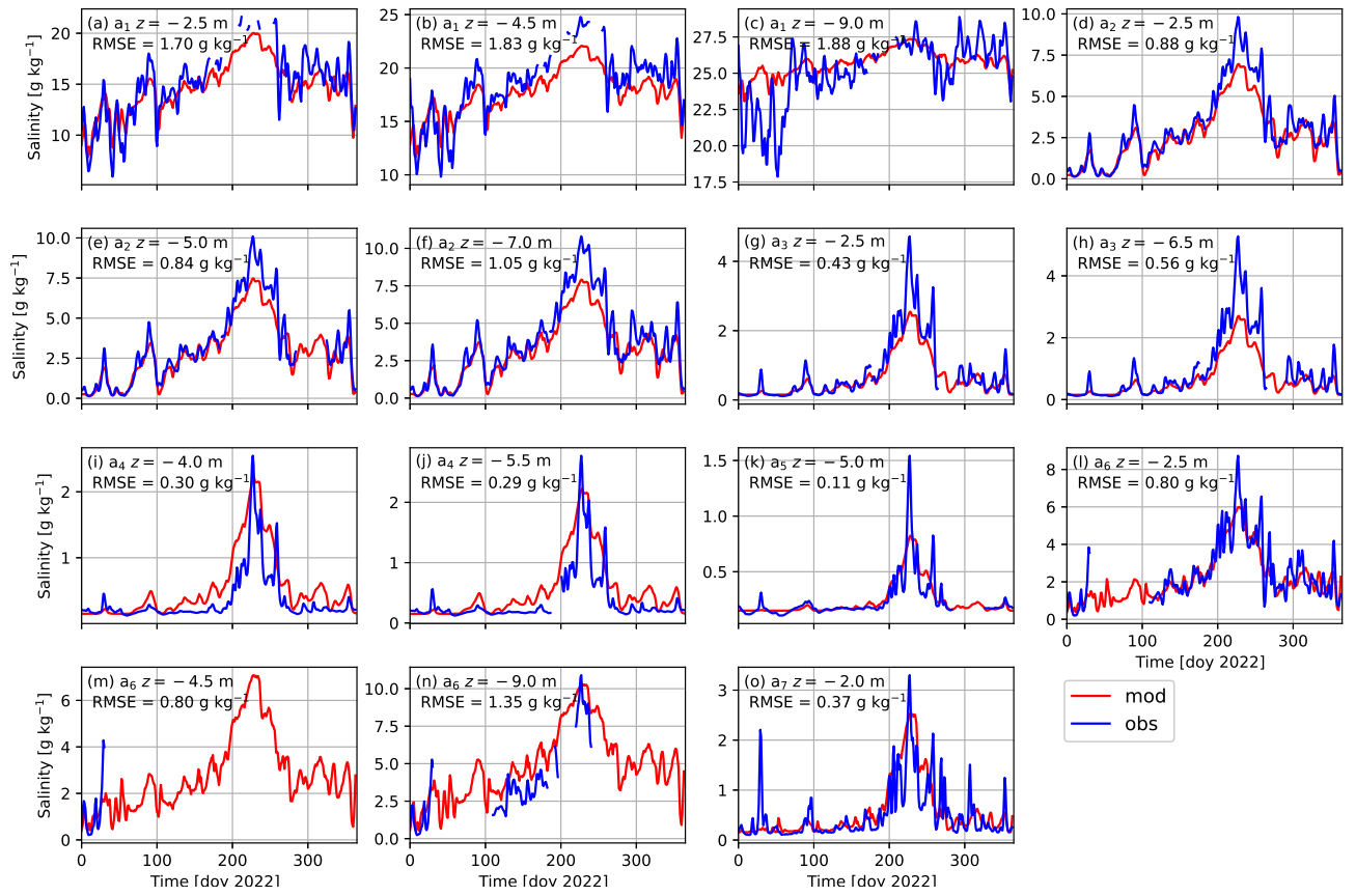
Figure S1. Observed (blue) and modelled (red) tidally averaged salinity time series for the year 2022 for different observation stations in the Rhine-Meuse Delta. Locations of the stations are indicated in Fig. 1 in the main text.
