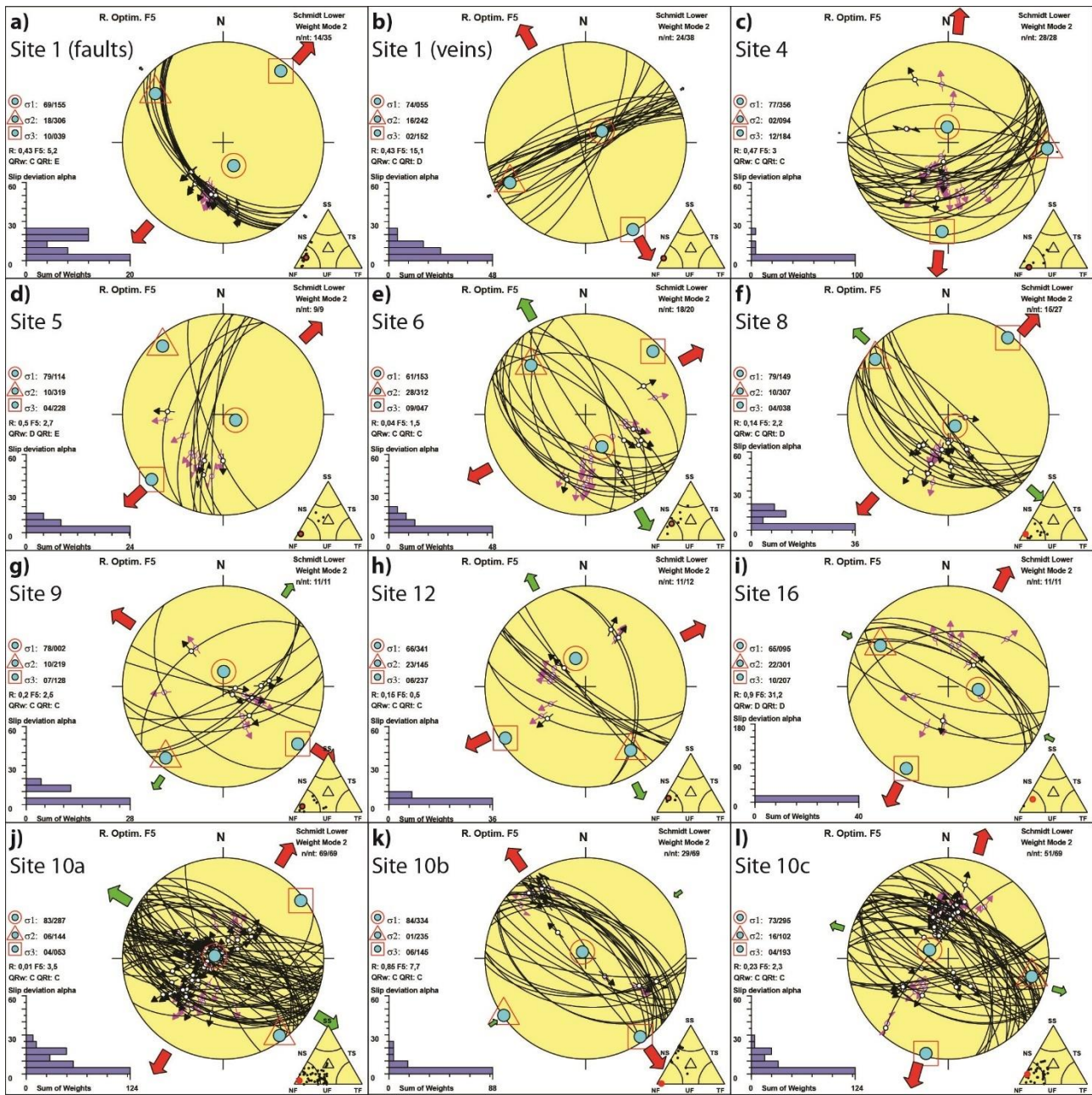
235 Figure 7: Paleostress tensors calculated from the inversion of fault-slip data using the Win-Tensor software (Delvaux, 1993). Stereograms are Schmidt lower hemisphere projections. In the stereograms, black arrows represent the measured hanging wall slip vector on a fault plane; purple arrows represent the theoretical optimal slip vector on a fault plane with respect to the computed paleostress tensor. Site numbers refer to numbers of the structural stations in Fig. 3. In the Frohlich triangles, NF: pure normal faulting; TF: pure reverse faulting; SS: pure strike slip faulting; NS: transtension; TS: transpression; UF: radial extension.
