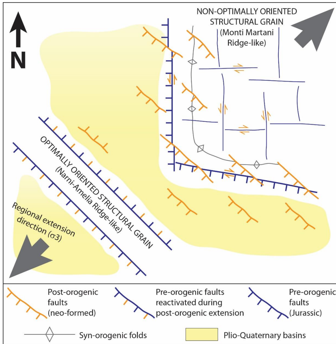
525 Figure 16: conceptual model for the development of post-orogenic extensional faults in the Monti Martani area. Optimally oriented structures are preferentially reactivated during post-orogenic extension and favor the formation of longer seismogenic normal faults. By contrast, a non-optimally oriented inherited structural grain with respect to the regional extensional stress field favors the activation of shorter, neo-formed normal faults which are ca. perpendicular to the regional extension direction.
