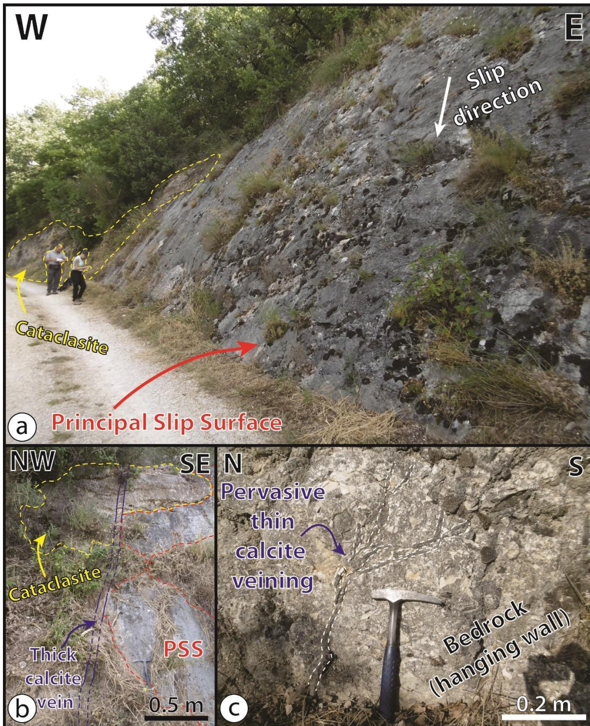
270 Figure 8: Extensional fault surface exposed in the Viepri area (site 1 in Fig. 3) (a) with examples of the calcite veins network hosted in the cataclasite (b) and the hanging wall (c). Structural measurements from this site are reported in stereonet n. 1 in Fig. 6.
