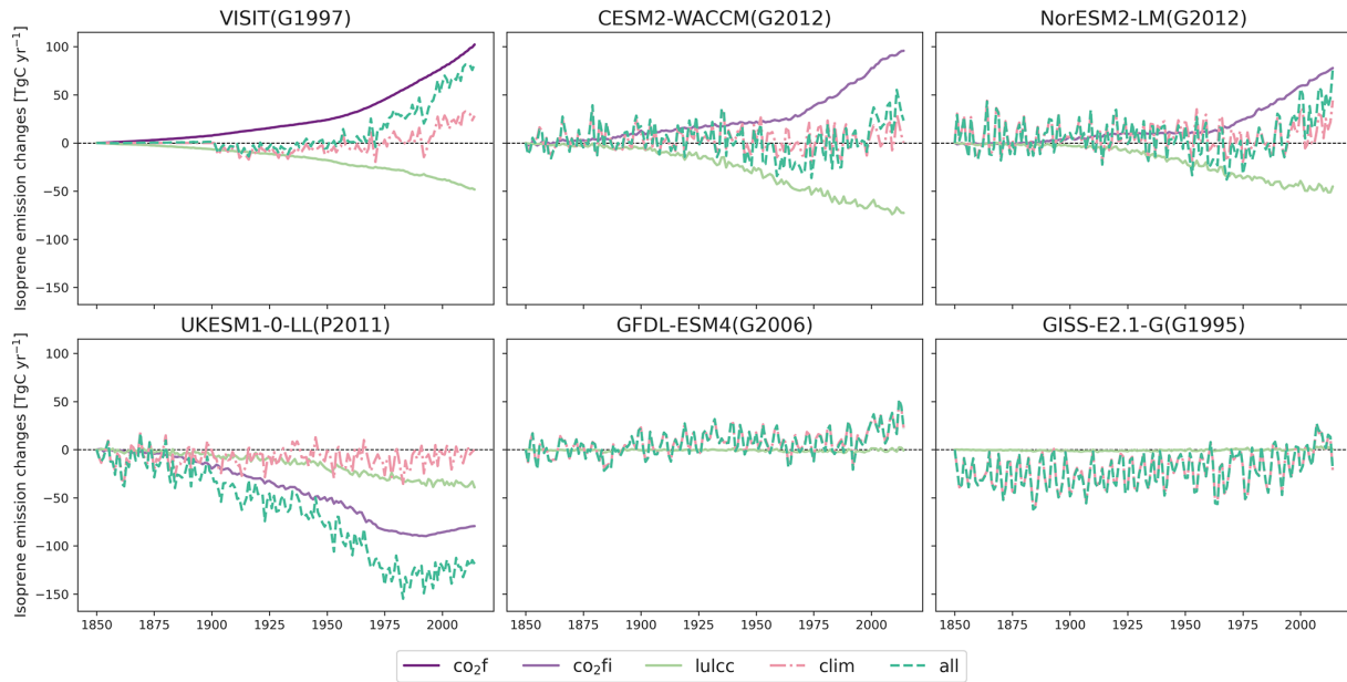
Figure 6. Effects of drivers on global isoprene emissions during 1850–2014: CO 2 (co 2 f, CO 2 fertilization only; co 2 fi, combined CO 2 fertilization and inhibition), land use and land cover change (lulcc), climate (clim), and the combination of three drivers (all). These effects were calculated as the difference in isoprene emission simulations between fixed and varied states for each driver, details of which are described in Sect. 2.3.1.
