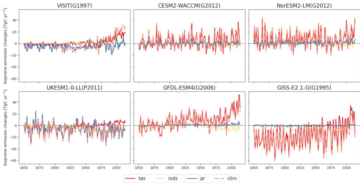
Figure 8. Effects of climate factors on global isoprene emissions during 1850–2014: temperature (tas), shortwave radiation (rsds), precipitation (pr), and total climate factors (clim).
