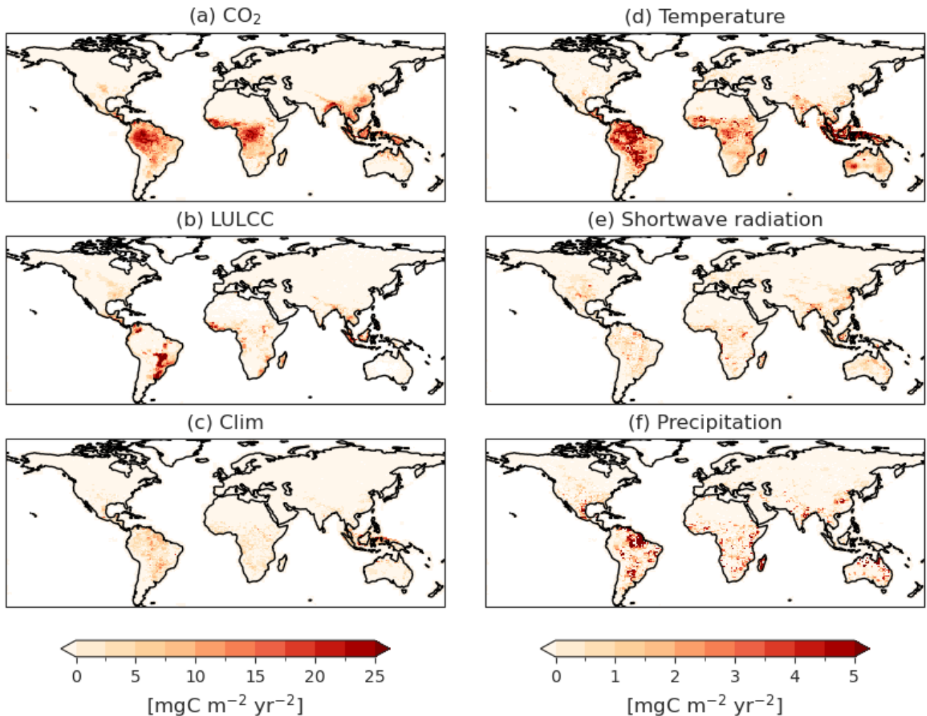
Figure 1414. Inter-model spreads of isoprene emission trends attributable to the following: (a) CO 2 ; (b) LULCC; (c) combined effects of three climate factors; and (d–f) the respective climate factors of temperature, shortwave radiation, and precipitation.
