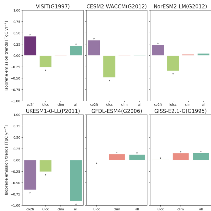
475 Figure 7. Attribution of global isoprene emission trends during 1850–2014 attributable to each driver ( \text{co2f}/\text{co2fi} , \text{lulcc} and \text{clim} ) and the combination of three drivers ( \text{all} ). Asterisks denote that the trend is significant, with p < 0.05 .
