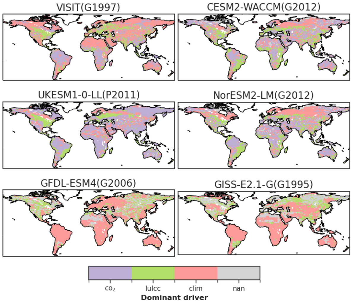
530 Figure 11. Dominant driver of isoprene emission trends between 1850 and 2014. For each grid, the factor generating the absolute largest trend is selected as the dominant driver. “nan” denotes no significant trend in isoprene emissions because of any factor. It is noteworthy that GFDL-ESM4(G2006) and GISS-E2.1-G(G1995) do not include the CO 2 effects.
