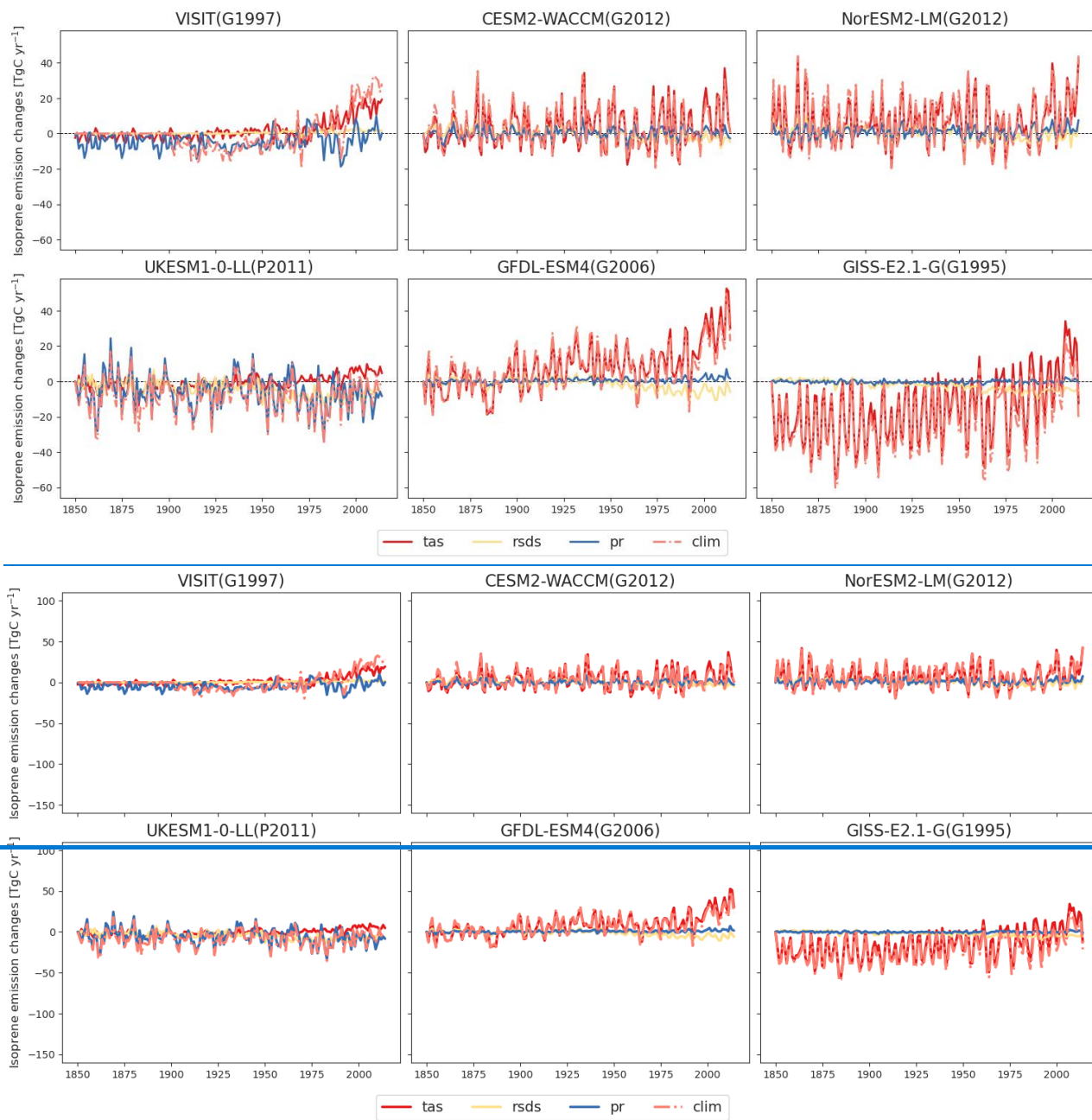
Figure 8. Effects of climate factors on global isoprene emissions during 1850–2014: temperature (tas), shortwave radiation (rsds), precipitation (pr), and total climate factors (clim).
