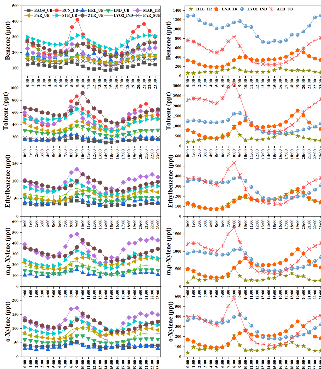
365 Figure 3. Diel variations of hourly average BTEX mixing ratios for 14 of the 22 studied sites, presented 370 in local time over the entire sampling period for each site. Please note that the two vertical axis of each 375 compound span different ranges of mixing ratios.
