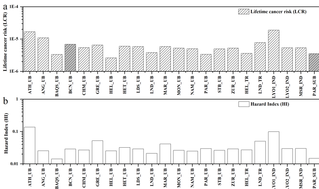
Figure 6. The lifetime cancer risk (LCR) values for the carcinogenic risk of benzene and ethylbenzene and hazard index (HI) for the carcinogenic risk of benzene, toluene, ethylbenzene, m,p-xylene, o-xylene through inhalation for individuals at all sites. Please note that the LCR values of BCN_UB and PAR_SUB have only been calculated with benzene data (marked gray), and HI values of BAQS_UB
