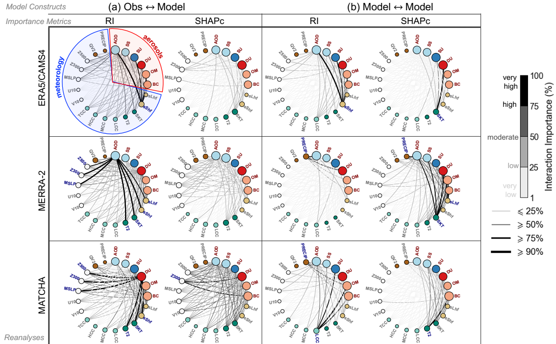
Figure 4. Strength of aerosol-meteorology interactions on snow within each reanalysis for different metrics and constructs. Network diagrams depicting the interaction importance/strength for both model constructs, Obs-Model (a) and Model-Model (b) using the relative importance (RI) and Shapely contribution (SHAPc) importance metrics of predictors within aerosol-meteorology interactions onto snow (AMI) in low snow-cover regions during the late snowmelt period (May-July). The nodes denote each predictor, while the lines (edges) denote the interaction importance on snow between the aerosol and meteorology variables, with their weights denoting the strength of the importance (1 to 100%, very low-low for \leq 25\% , low-moderate for 25% to 50%, moderate-high for 50% to 75%, and high-very high for \geq 75\% shown in the color bars). The node sizes differ between AER and MET predictors based on their weighted degree (number of edge connections, see Appendix A). The variable abbreviations at the nodes include the following aerosol variables; AOD for total AOD at 550 nm; SU for surface sulphate mixing ratio; SS for surface sea-salt mixing ratio; DU for surface dust mixing ratio; OM for surface organic matter mixing ratio and BC for surface black carbon mixing ratio. For meteorology, the abbreviations are as follows, PRECIP for daily accumulated precipitation; QV2 for specific humidity at 2 m; Z500 and Z300 for geopotential height at 500 and 300 hPa; U10 and V10 for zonal and meridional winds at 10 m; MSLP for mean sea level pressure; MCC, TCC, LCC and HCC for medium, total, low and high cloud cover fraction; T2 for temperature at 2 m; SKT for skin temperature; sShf and sLhf for surface sensible and latent heat flux; and finally ELEV for elevation. Details about these predictors can be found in Supplementary Table 2.
