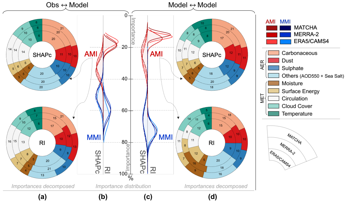
Figure 2. Importance of aerosol-meteorology interactions on snow and their constituent variables. Distributions of importance metrics (b-c), relative importance (RI), and Shapely contribution (SHAPc) for aerosol-meteorology (AMI) and meteorology-meteorology (MMI) interactions on snow shown for the Obs-Model (b) and Model-Model (c) construct for the three reanalyses. AMI's importance on snow is further decomposed into nine subgroups of predictors (four aerosol/AER and five meteorology/MET subgroups), which are shown in the donut pie-plots for the Obs-Model (a) and Model-Model (d) constructs for both RI (bottom row) and SHAPc (top row). The innermost ring shows the contribution of each subgroup to AMI's importance on snow from the ERA5-CAMS4 reanalysis, followed by MERRA-2 and MATCHA in the outermost ring.
