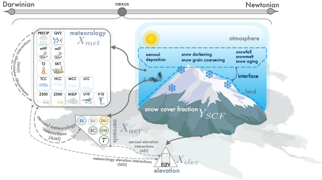
Figure 1. Schematic describing an integrated approach to assess interactions at the atmospheric-cryospheric (land) interface over High Mountain Asia. The Darwinian view focuses on the individual predictors (shown by the 22 icons grouped by meteorology, aerosols, and elevation) that drive snowmelt while the Newtonian view emphasizes emerging patterns and physics-based processes driving snowmelt (shown in the interface between the atmosphere and land). This study lies at the nexus of both perspectives where we assess the sensitivity of snow cover fraction to the interactions between aerosols and meteorology variables at the interface (aerosol-meteorology interactions or AMI) on snow. Likewise, we also consider meteorology-meteorology interactions (MMI) on snow, aerosol–elevation interactions onto snow (AEI), and meteorology–elevation interactions (MEI) on snow. Abbreviations of the individual predictors are mentioned in the acronym section (Appendix B). The overlaid map of Asia is taken from FreeVectorMaps at https://freevectormaps.com/world-maps/asia/WRLD-AS-02-4001?ref=atr .
