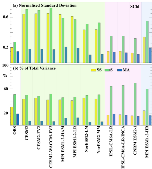
Figure 3: Variability across timescales for SChI (a) Normalised standard deviation of SChI from observation and CMIP6 historical models. Standard deviation at each grid point is normalised by the mean over each grid. (b) Percentage of SChI variance explained by each component (sub-seasonal, seasonal and multi-annual) for observations and CMIP6 historical models. Shading represents the different model groups described in Section 3.2, with green for Group 1, pink for Group 2, and blue for Group 3.
