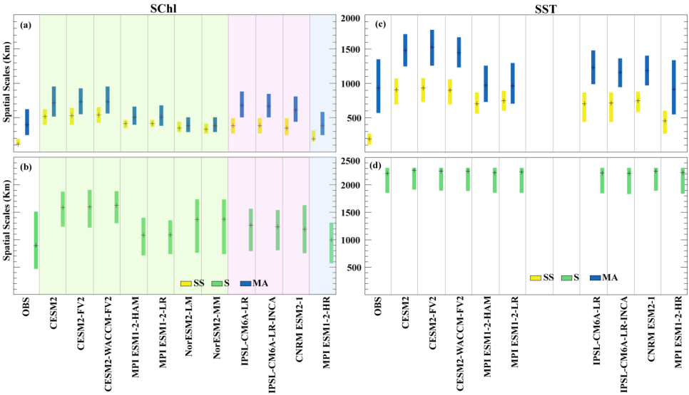
330 Figure 5: Spatial scales corresponding to each timescales: The spatial scales associated with sub-seasonal (yellow), seasonal (green) and multi-annual (blue) variations of SchI (a,b) and SST (c,d). The black line within each box denotes the median. Shading in panel a and b represents the different model groups described in Section 3.2, with green for Group 1, pink for Group 2, and blue for Group 3.
