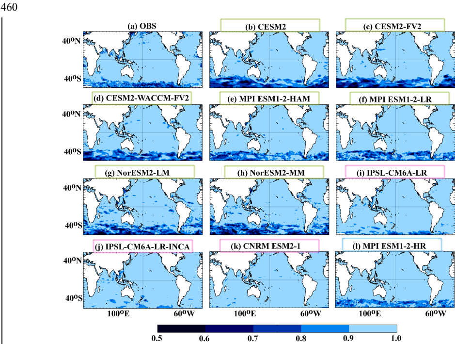
Figure 8: Annual mean low-frequency index for SchI , which is defined as the correlation square between annual mean and annual mean of the multi-annual component. When the index is close to one, year-to-year fluctuations in the annual mean reflect low-frequency variability. The value of the index decreases as high-frequency variability contributes more to year-to-year variations. Coloured boxes for the model names represent the different model groups described in Section 3.2, with green for Group 1, pink for Group 2, and blue for Group 3.
