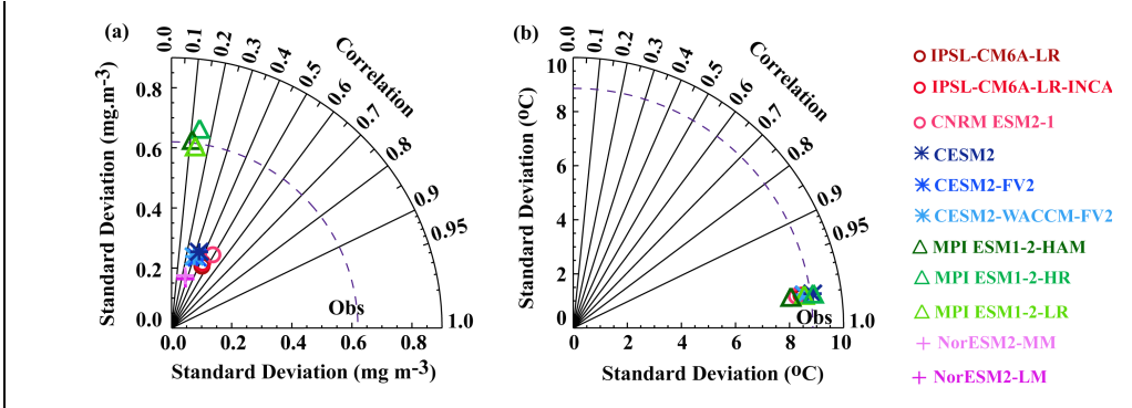
Figure 2: Evaluation of the mean spatial distribution: Taylor diagram for the annual mean (a) SCHl and (b) SST over the years 1998-2014 and domain 60^{\circ}\text{N} - 60^{\circ}\text{S} . The dashed curve represents the standard deviation of the observational data.
