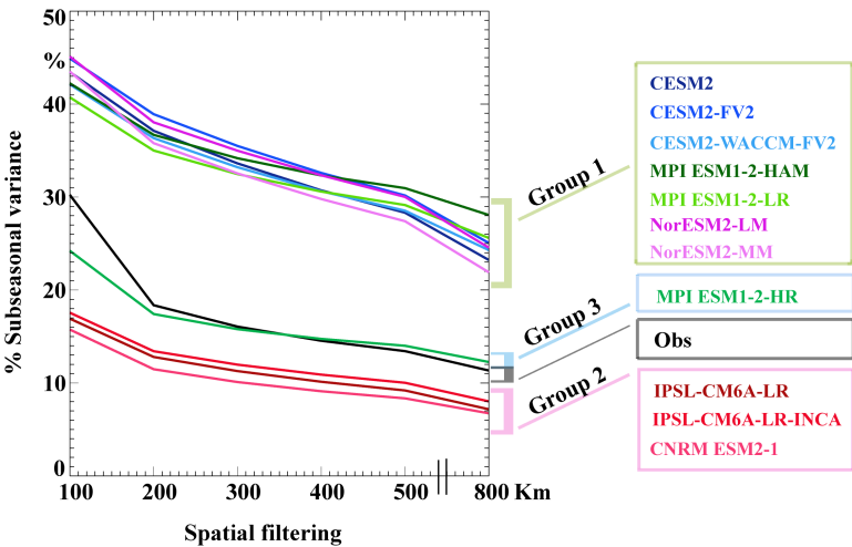
380 Figure 6: Sub-seasonal variance across spatial scales: Percentage of total SChI variance explained by sub-seasonal variability after applying a spatial smoothing of varying scale from 100 km to 800 km to the SChI data. Coloured boxes for the model names represent the different model groups described in Section 3.2, with green for Group 1, pink for Group 2, and blue for Group 3.
