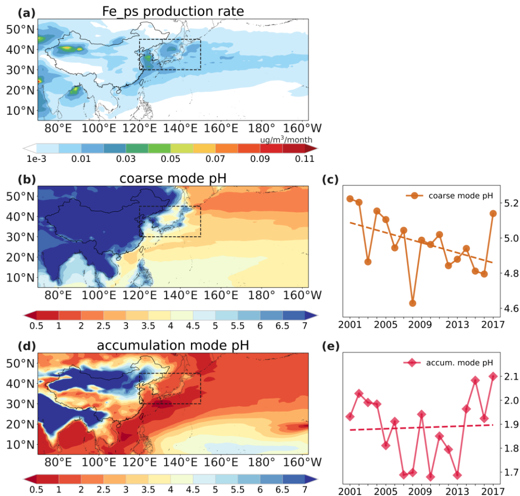
390 Figure 7: Spatial distributions of surface dust soluble iron production rate from proton-promoted processing (a), surface coarse mode aerosol pH (b), and surface accumulation mode aerosol pH (d) averaged of 2001-2017 springs. Temporal variations of surface coarse mode pH (c) and accumulation mode pH (e) over high production rate area (30-45°N, 120-150°E) averaged of 2001-2017 springs.
