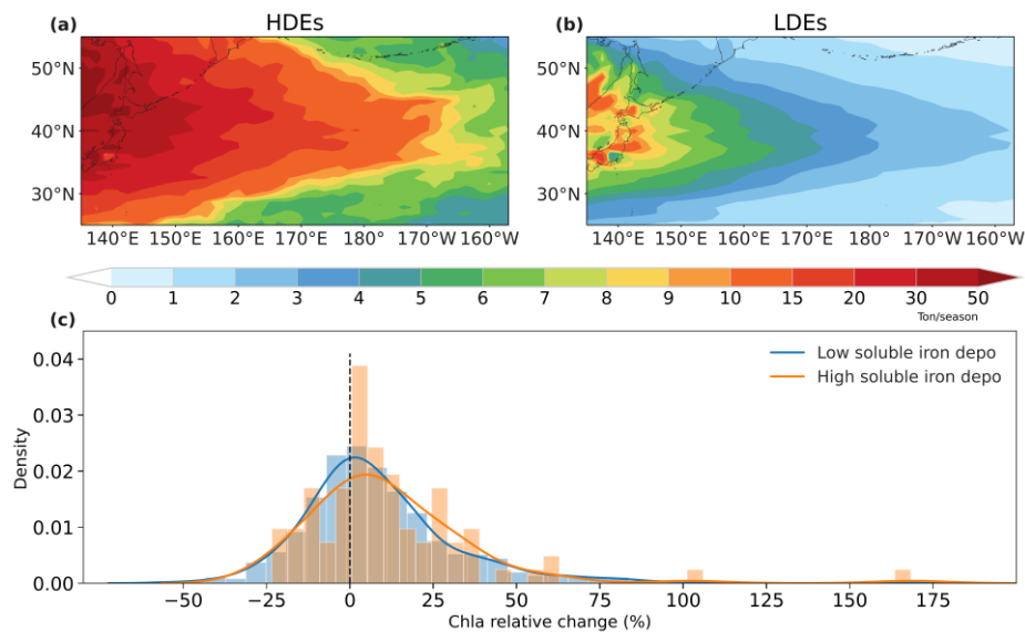
510 Figure 10: Spatial distributions of selected high (a) and low (b) soluble iron deposition averaged of 2001-2017 springs. (c) probability distribution function of relative changes in chlorophyll-a averaged over NWP after high (orange) and low(blue) deposition events.
