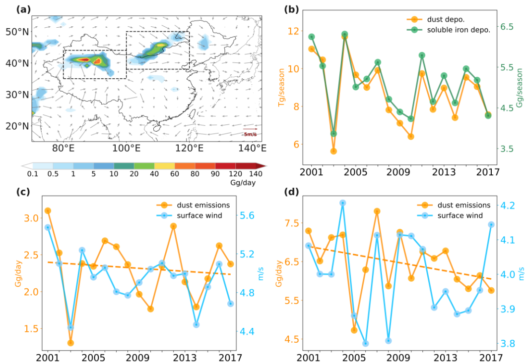
375 Figure 6: (a) Spatial distributions of dust emission flux and surface wind over Eastern Asia during 2001-2017 springs. (b) Temporal variations of dust (yellow) and soluble iron (green) deposition to Northwest Pacific (30-50N, 140E-160W). (c, d) Temporal variations of dust emission flux (yellow) and surface wind (blue) over the Gobi dust source (38-50N, 100-120E) and Taklamakan dust source (35-43N, 80-100E) on average of 2001-2017 springs.
