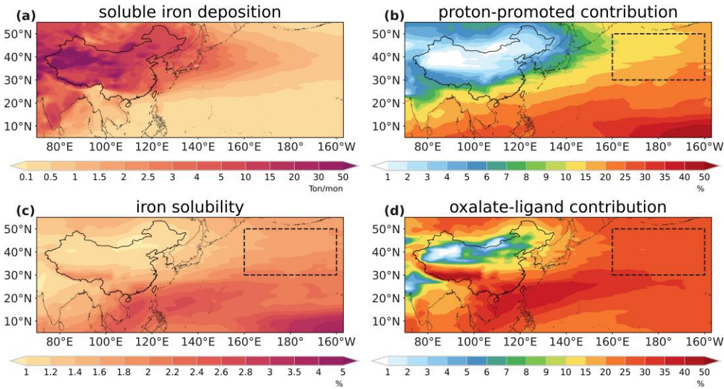
305 Figure 4: Spatial distributions of (a) soluble iron deposition, (c) iron solubility, (b) proton-promoted relative contributions to soluble iron deposition, and (d) oxalate-promoted contributions to soluble iron deposition on average of 2001-2017 springs.
