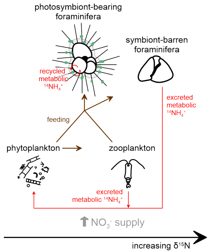
Figure 6. Proposed interactions and processes influencing planktic foraminifera-bound nitrogen isotopes (FB-δ 15 N) in relation to symbiotic status and food sources. Symbiont-barren foraminifera, or those hosting symbionts other than dinoflagellates, record elevated FB-δ 15 N relative to their food source, as with typical zooplankton. In contrast, symbiont-bearing foraminifera exhibit lower FB-δ 15 N values due to their association with photosymbionts, which internally reassimilate the low-δ 15 N metabolic ammonium (NH 4 + ) from the foraminiferal host through photosynthesis, preventing or reducing the δ 15 N elevation that typically results from heterotrophy.
