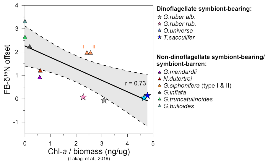
Figure 7. Chlorophyll- a concentrations in living planktic foraminifera vs. FB- \delta^{15}\text{N} offsets between dinoflagellate-bearing and other non-dinoflagellate-bearing foraminifera. Chlorophyll- a /biomass values were measured in foraminifera collected in the central and western Pacific Ocean and the tropical eastern Atlantic Ocean across different seasons (Takagi et al., 2019) and compared to the median of the FB- \delta^{15}\text{N} offsets in our core top compilation (Fig. 5, S5, Table S2).
