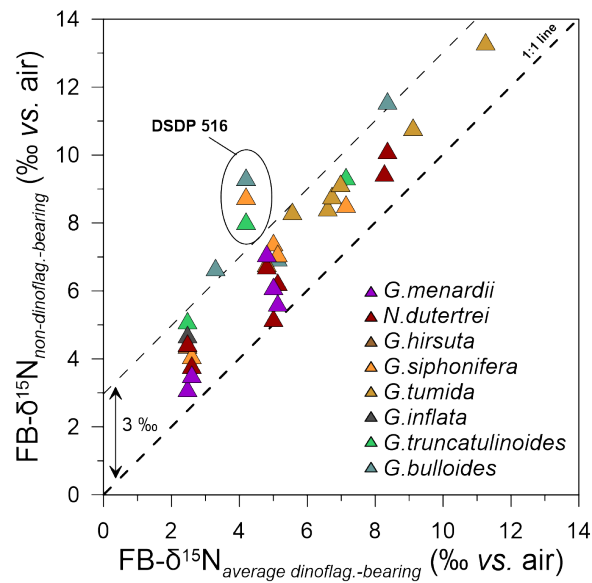
Figure 8. FB- \delta^{15}\text{N} offsets between non-dinoflagellate-bearing foraminifera vs dinoflagellate-bearing foraminifera (the average of G. ruber albus , T. sacculifer and O. universa ), with DSDP Site 516 indicated having uniquely high FB- \delta^{15}\text{N} offsets. DSDP Site 516 exhibits stronger ^{15}\text{N} enrichment for non-dinoflagellate-bearing foraminifera than other sites from the global core top compilation (see Table S1 and Figure S5).
