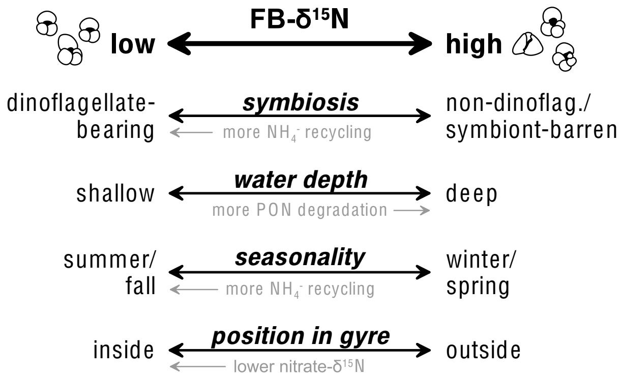
540 Figure 10. Proposed different processes affecting \text{FB-}\delta^{15}\text{N} at DSDP Site 516. Shallow-dwelling, summer-blooming, dinoflagellate-bearing foraminifera located within the oligotrophic gyre record generally lower \text{FB-}\delta^{15}\text{N} values than symbiont-barren or foraminifera hosting symbionts other than dinoflagellates that live generally in a deeper depth habitat, bloom during winter/spring season and/or live outside oligotrophic gyres.
