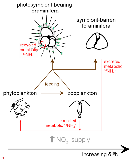
Figure 6. Proposed interactions and processes influencing planktic foraminifera-bound nitrogen isotopes (FB- \delta^{15}\text{N} ) in relation to symbiotic status and food sources. Symbiont-barren foraminifera, or those hosting symbionts other than dinoflagellates, record elevated FB- \delta^{15}\text{N} relative to their food source, as with typical zooplankton. In contrast, symbiont-bearing foraminifera exhibit lower FB- \delta^{15}\text{N} values due to their association with photosymbionts, which internally reassimilate the low- \delta^{15}\text{N} metabolic ammonium ( \text{NH}_4^+ ) from the foraminiferal host through photosynthesis, preventing or reducing the \delta^{15}\text{N} elevation that typically results from heterotrophy.
