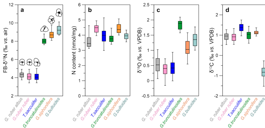
Figure 3. Box plots of species-specific nitrogen, carbon and oxygen isotopes at DSDP Site 516. (a) Species-specific FB-δ¹⁵N values averaged over the last 160 ka for G. bulloides (turquoise), G. siphonifera (orange), G. truncatulinoides (green), T. sacculifer (blue), G. ruber ruber (pink) and G. ruber albus (grey). (b) N content for each species. (c & d) Species-specific δ¹⁸O and δ¹³C, respectively.
