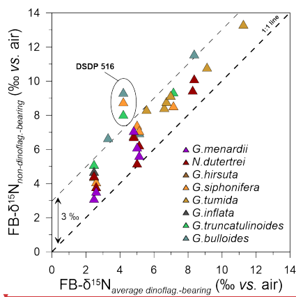
920 Figure 8. FB- \delta^{15}\text{N} offsets between non-dinoflagellate-bearing foraminifera vs dinoflagellate-bearing foraminifera (the average of G. ruber albus , T. sacculifer and O. universa ), with DSDP Site 516 indicated, having uniquely high FB- \delta^{15}\text{N} offsets. DSDP Site 516
