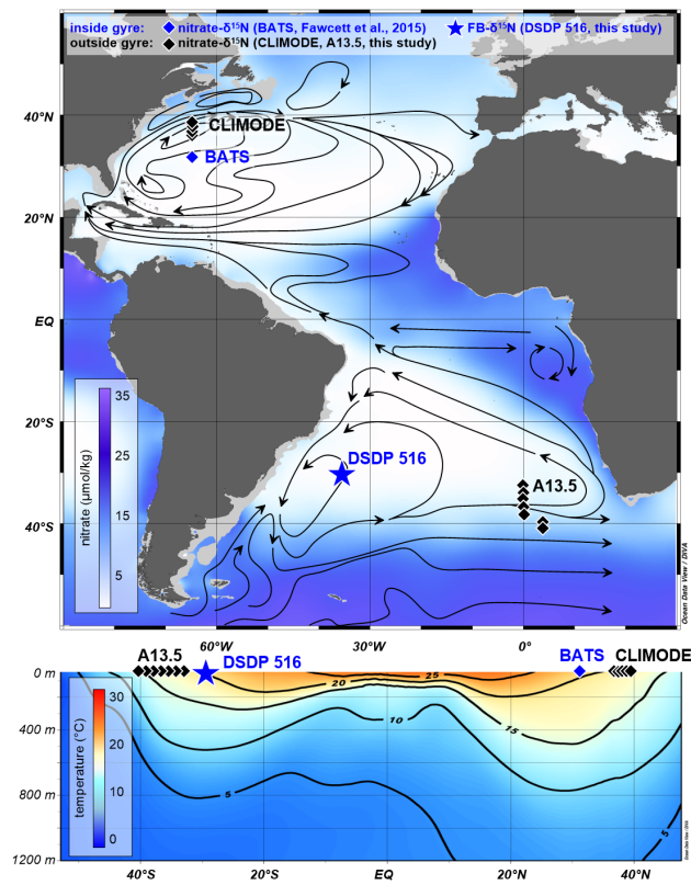
Figure 1. Oceanographic context for DSDP Site 516. (a) Nitrate map (in μmol/kg) at 100 m water depth with sample location DSDP Site 516 for FB-δ¹⁵N (this study) and nitrate δ¹⁵N profiles from CLIMODE (this study), BATS (Fawcett et al., 2015) and A13.5 (this study). Main surface currents and oceanographic fronts modified from (Peterson and Stramma, 1991; Wefer et al., 1996) and (Schmitz Jr. and McCartney, 1993) (b) Mean annual temperature cross section. Map and cross section generated with Ocean Data View and data set from World Ocean Atlas 18 (Garcia et al., 2013; Schlitzer, 2015).
