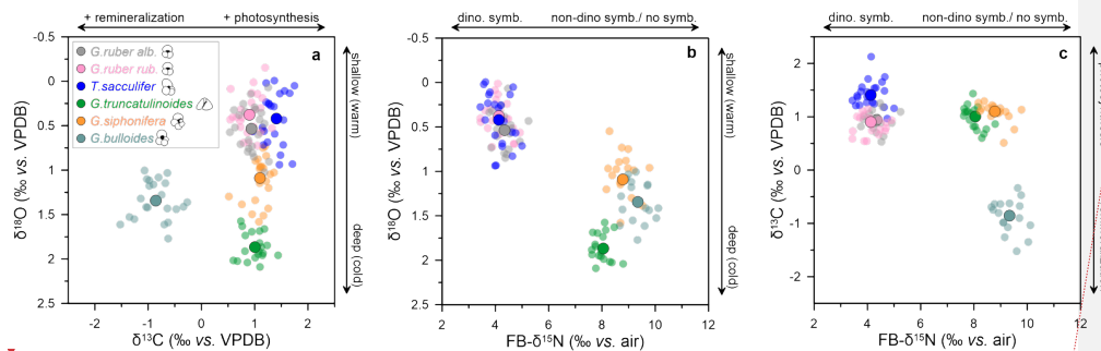
Figure 4. Relationships between oxygen, carbon and nitrogen isotopes. Interspecies comparison between G. ruber ( albus and ruber ), T. sacculifer , G. truncatulinoides , G. siphonifera and G. bulloides at DSDP Site 516. Arrows indicate distinction between shallow (warm) vs. deep (cold) dweller, remineralization vs. photosynthesis in the water column and non-dinoflagellate bearing/non-symbiotic vs. dinoflagellate bearing foraminifera.
