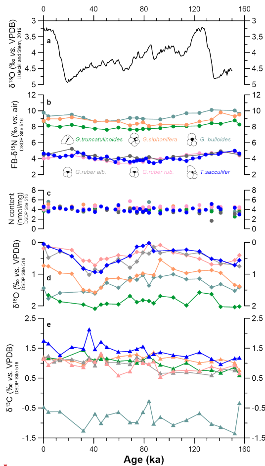
Figure 2. 160 kyr time series of species-specific nitrogen, carbon and oxygen isotopes at DSDP Site 516. (a) benthic foraminifera \delta^{18}\text{O} stack (Lisiecki and Stern, 2016). MIS = Marine Isotope Stages. (b) Species-specific FB- \delta^{15}\text{N} measured at DSDP 516 for G. bulloides (turquoise), G. siphonifera (orange), G. truncatulinoides (green), T. sacculifer (blue), G. ruber ruber (pink), and G. ruber albus (grey). (c) N content for each species. (d) Species-specific calcite- \delta^{18}\text{O} and (e) calcite- \delta^{13}\text{C} .
