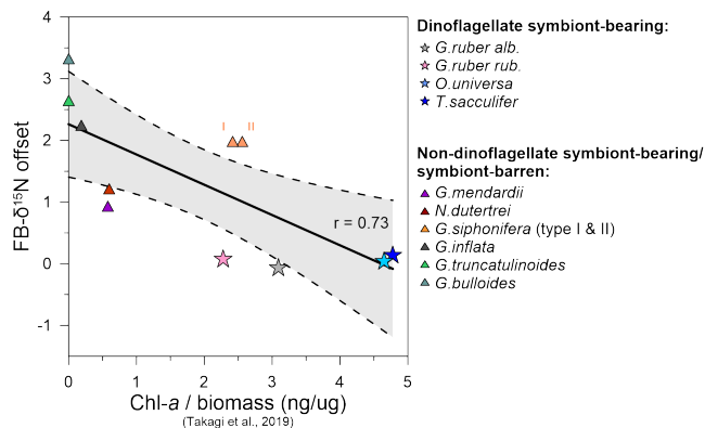
915 Figure 7. Chlorophyll- a concentrations in living planktic foraminifera vs. FB- \delta^{15}\text{N} offsets between dinoflagellate-bearing and other non-dinoflagellate-bearing foraminifera. Chlorophyll- a /biomass values were measured in foraminifera collected in the central and western Pacific Ocean and the tropical eastern Atlantic Ocean across different seasons (Takagi et al., 2019) and compared to the median of the FB- \delta^{15}\text{N} offsets in our core top compilation (Fig. 5, S5, Table S2).
