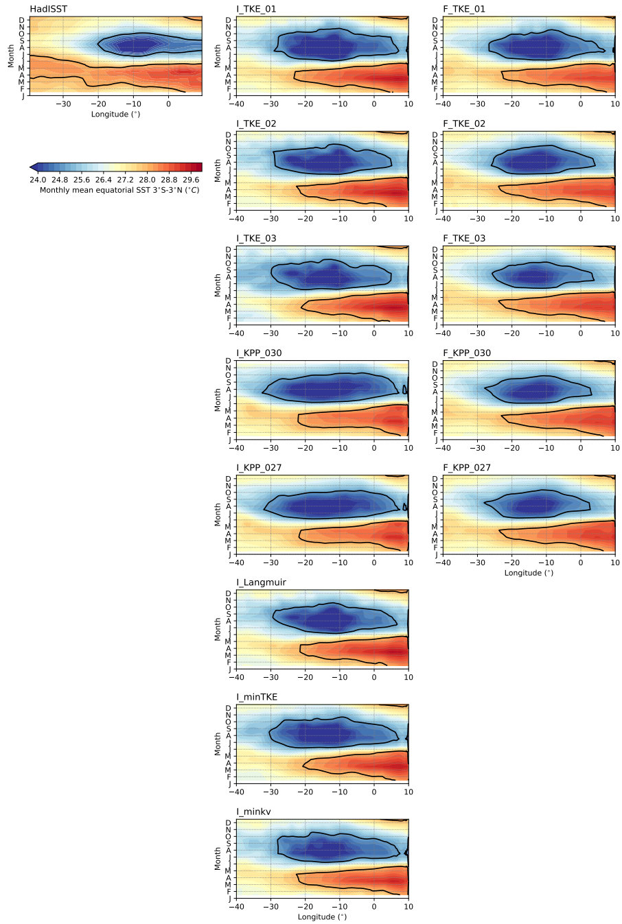
Figure 7. Hovmoeller plots of monthly mean SST in 2015 averaged between 3^{\circ} S and 3^{\circ} N for the HadISST dataset (left), the ICON-O simulations (center) and the FESOM simulations (right). The black contours correspond to 25^{\circ} and 28^{\circ} C.
