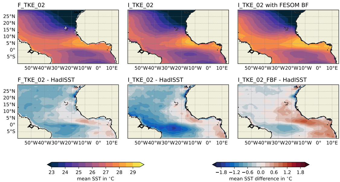
Figure 18. Effect of exchanging the forcing bulk formulae in ICON-O on the 2015 annual mean mixed-layer depth sea surface temperature. The upper three panels show the 2015 annual mean SST from the FESOM TKE_02 run and the ICON-O TKE_02 run as well as the ICON-O TKE_02 run with the bulk formulae used in FESOM. The lower panels show from the same three runs the difference to 2015 annual mean SST from HadISST as shown in Figure 4.
