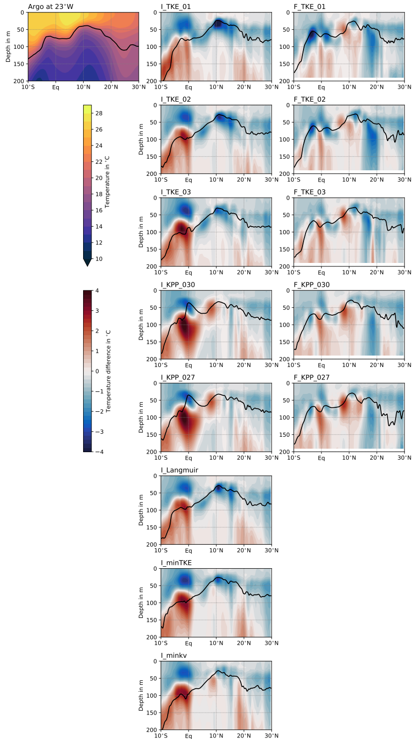
Figure 10. Vertical section along 23^\circ\text{W} of 2015 annual mean temperature from (shading) and the 2015 ,from annual mean thermocline depth (black contour) for Argo float data as well as (top left panel), and difference to Argo for FESOM and ICON-O. The temperature sections have been averaged between 24^\circ\text{W} and 22^\circ\text{W} .
