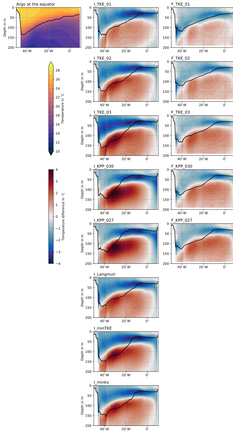
Figure 9. Vertical section along the equator of 2015 annual mean temperature from (shading) and the 2015 -from- annual mean thermocline depth (black contour) for Argo float data as-well-as- (top left panel) and difference to Argo for FESOM and ICON-O. The temperature sections have been averaged between 1° S and 1° N.
