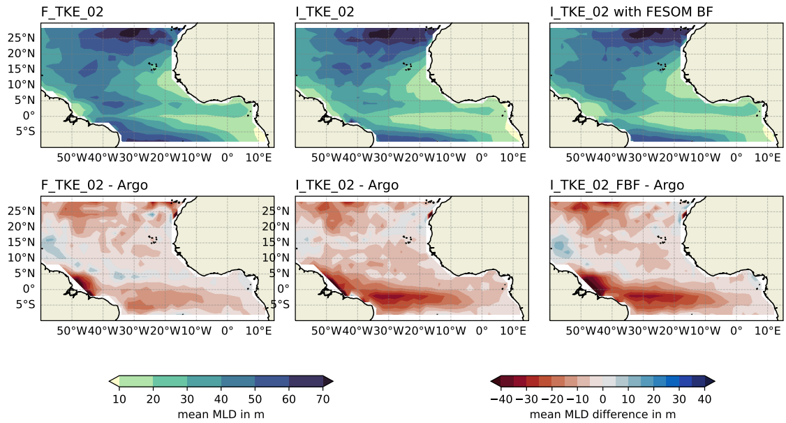
Figure 19. Effect of exchanging the forcing bulk formulae in ICON-O on the 2015 annual mean sea surface temperature mixed layer depth . The upper three panels show the 2015 annual mean MLD from the FESOM TKE_02 run and the ICON-O TKE_02 run as well as the ICON-O TKE_02 run with the bulk formulae used in FESOM. The lower panels show from the same three runs the difference to the mean MLD from Argo float data as shown in Figure 2.
