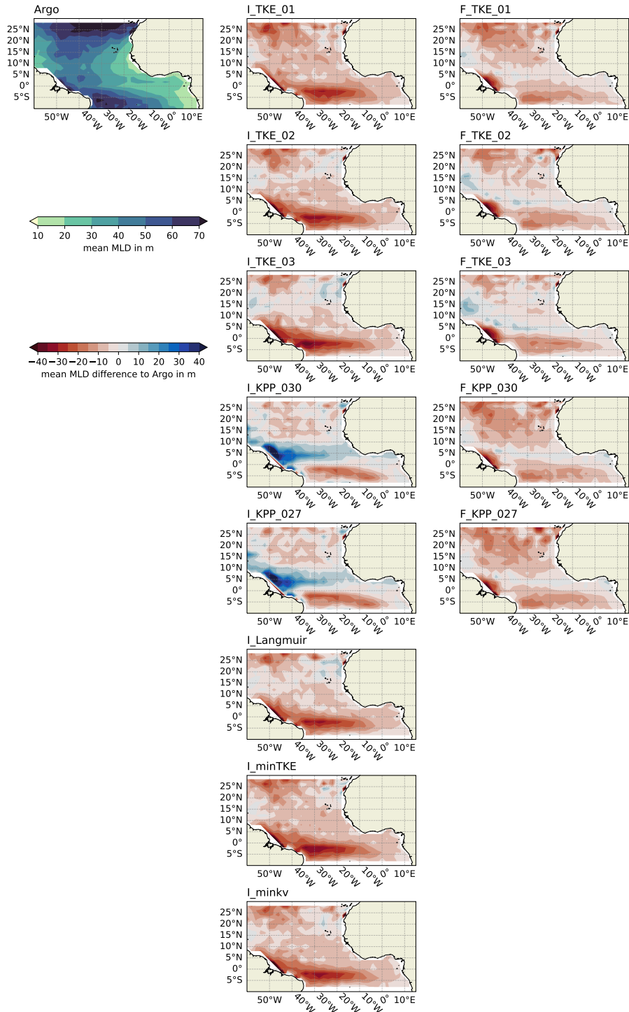
Figure 2. Difference in annual Annual mean mixed layer depth between FESOM and in 2015 for the different simulations of ICON-O runs and Argo float data in FESOM (centre and right panels) relative to the tropical Atlantic Ocean Argo climatology (top left panel).
