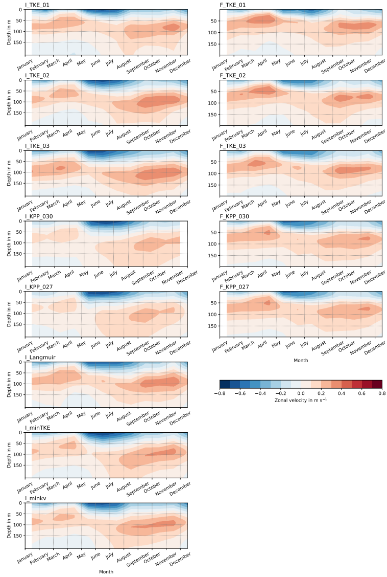
Figure 12. Hovmoeller plot of monthly-mean zonal velocity in 2015 as a function of depth at 23° W, where the cruise observations displayed in Figure 11 are located, averaged between 3° S and 3° N. The panels on the left are for the various ICON-O simulations and those on right for the FESOM simulations.
