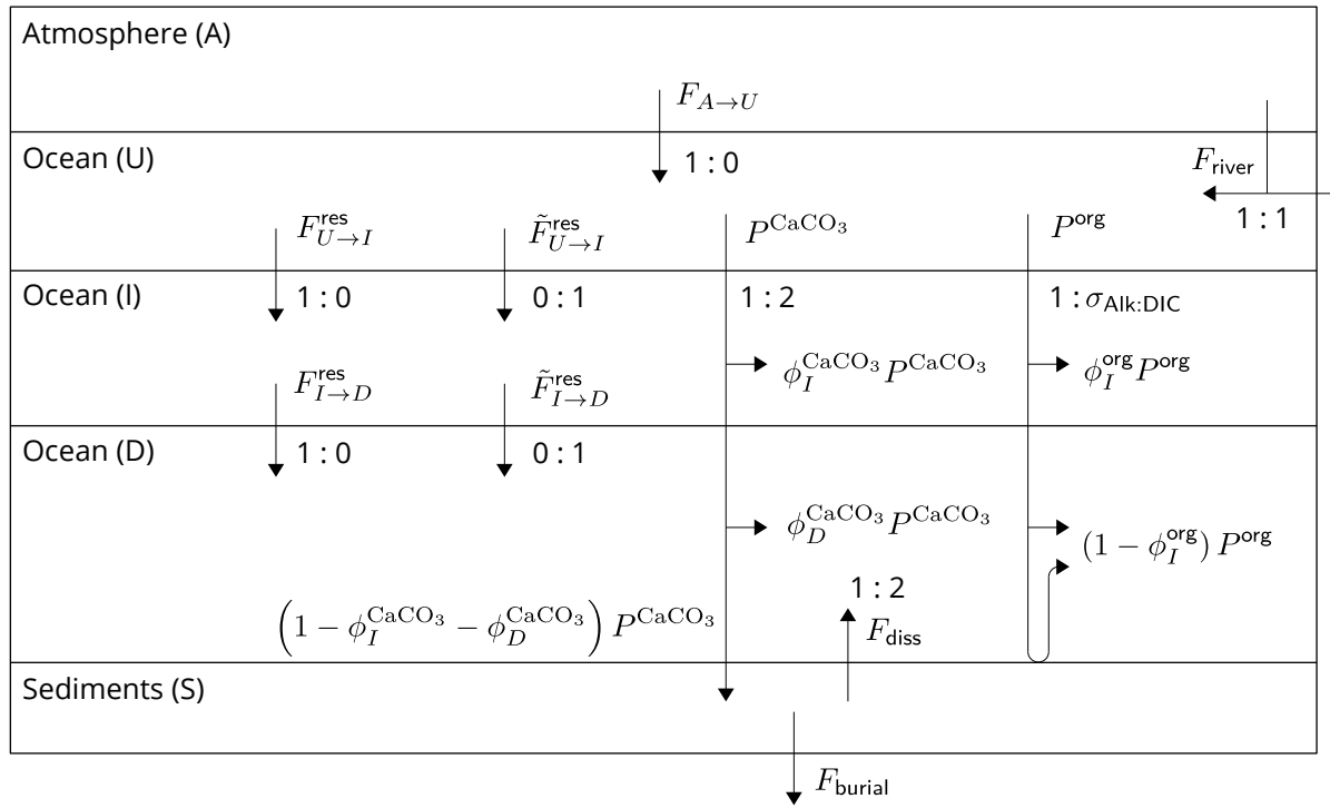
Figure 2. Schematic diagram of the DIC and Alk fluxes in SURFER v3.0. The ratios are ratios of DIC to alkalinity changes, i.e a : b ratio indicates that for a DIC change of a moles, there is an associated alkalinity change of b moles.
