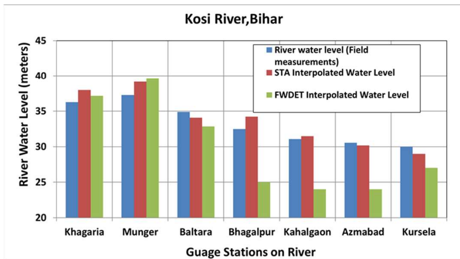
Figure.10. Comparison plots for water levels among field measured data, TSA and FWDET on all study areas
