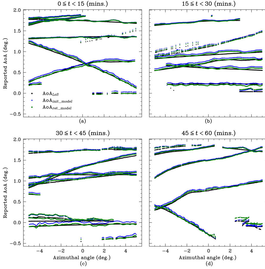
Figure 10. The LoS AoA as a function of azimuthal angle (where 0^\circ corresponds to the centre of the observational sector). The black points ( AoA_{LoS} ) indicate the LoS AoA derived from the decoded ADS-B transmissions. The blue points indicate the modelled LoS AoA ( AoA_{init\_model} ) determined from tracing rays through the initial (first-guess) refractivity profile. The green points indicate the modelled LoS AoA ( AoA_{ret\_model} ) determined from tracing rays through the retrieved (optimised) refractivity profile. The time period was between 08:36 and 09:36 UTC.
