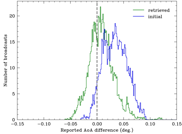
Figure 13. The distribution in the modelled LoS AoA difference for all observations using the initial (blue) and retrieved (green) refractivity profiles. The mean difference in the LoS AoA decreased from \sim 0.034^\circ to \sim 0.009^\circ for the initial and retrieved refractivity profiles respectively. The standard deviation in the LoS AoA difference increased from \sim 0.023^\circ to \sim 0.024^\circ for the initial and retrieved refractivity profiles respectively.
