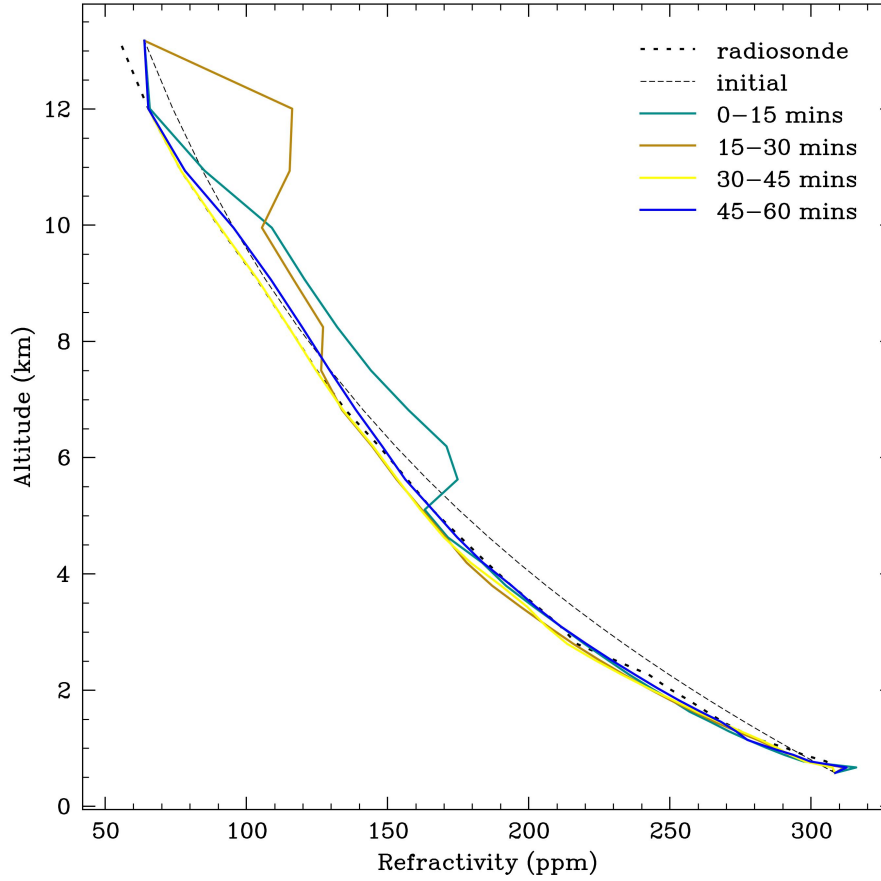
Figure 11. The 12:00 UTC 22 September 2023 Watnall radiosonde refractivity profile (dotted), retrieved (solid colour) and initial (dashed) refractivity profiles. The time period was between 08:36 and 09:36 UTC.
