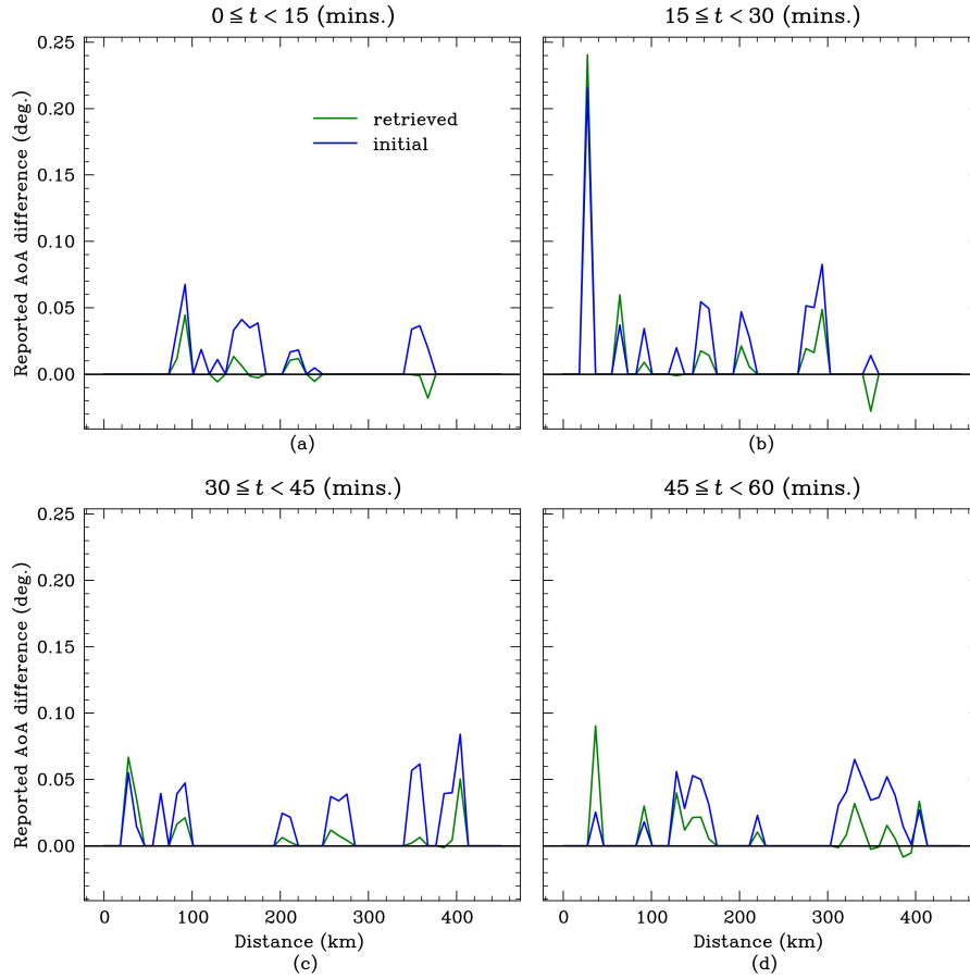
Figure 12. The difference between the AoA_{LoS} and AoA_{init\_model} (blue line) and the difference between the AoA_{LoS} and AoA_{ret\_model} (green line) as a function of distance. The time period was between 08:36 and 09:36 UTC.
