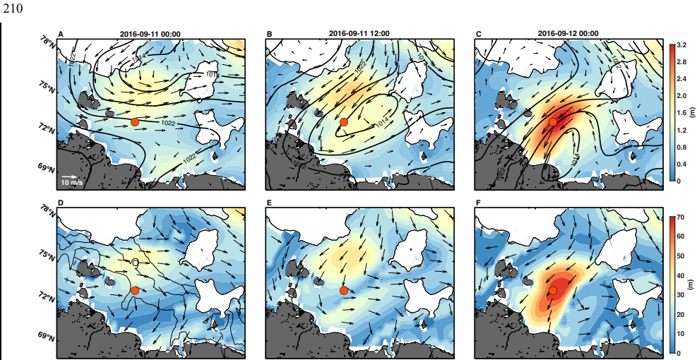
Figure 2: Distribution of significant wave height (top panel) and the wave length (bottom panel) every 12 hours during September 11-12. (a-c) The black contours represent sea level pressure in units of hPa. The arrows represent the 10 m wind field. The white area denotes sea ice extent, and the red asterisk marks the location of station LA-77-35. (d-f) Arrows indicate the wave direction. Thin black lines in (d-f) indicate 30 m, 50 m, and 100 m isobath, respectively.
