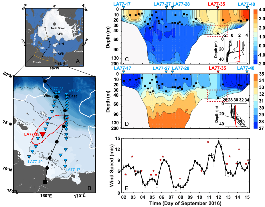
Figure 1: Observations in the East Siberian Sea (ESS).
