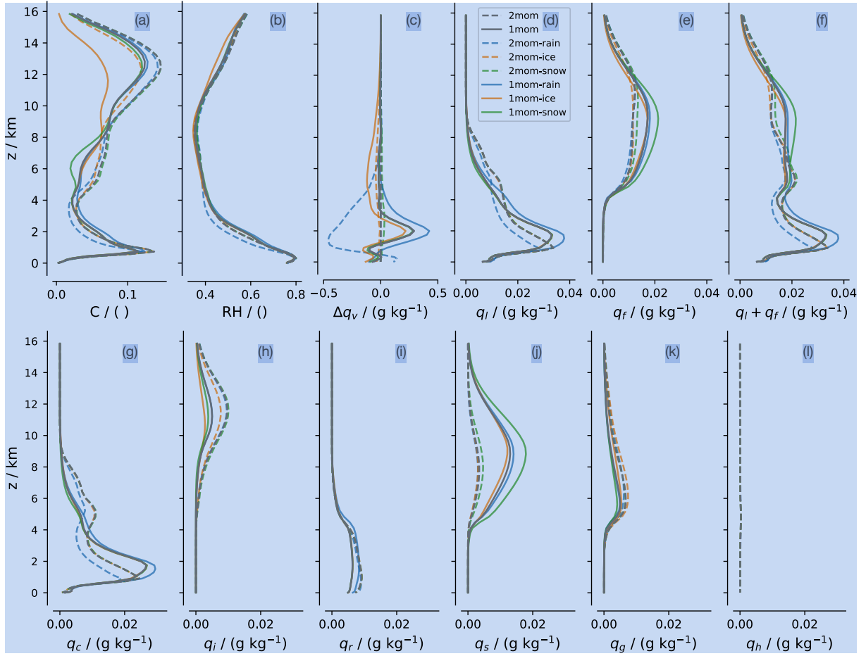
Figure 2. Tropical mean profiles of (a) cloud fraction, C ; (b) relative humidity, RH ; (c) specific water vapor mass as difference to 2mom; specific mass of (d) liquid condensate, q_l = q_c + q_r ; (e) frozen condensate, q_f = q_i + q_s + q_g + q_h ; (f) total condensate, q_l + q_f ; and for each hydrometeor category: (g) cloud water, q_c ; (h) cloud ice, q_i ; (i) rain, q_r ; (j) snow, q_s ; (k) graupel, q_g ; and (l) hail, q_h .
