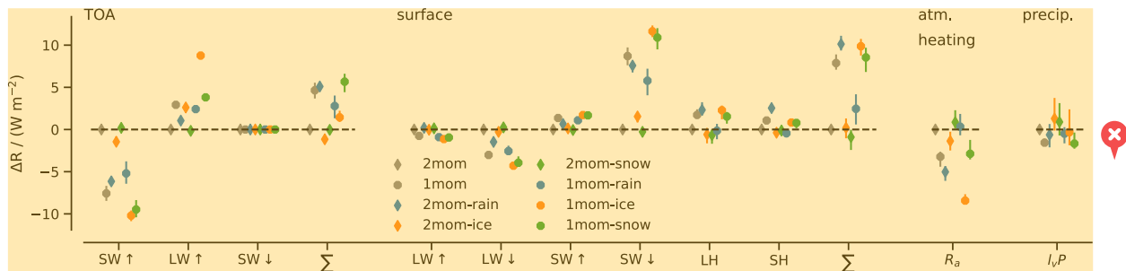
Figure D1. Same as Fig. 2.1 but for global means instead of the tropical belt.
