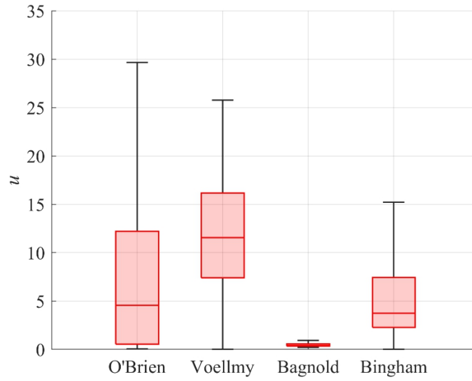
Figure 2. Uniform velocity boxplot distribution for the 4 rheological models used to perform Sobol sensitivity analysis ( h = 1 \text{ m} , \theta = 20^\circ ). For each graph the solid line represents the median value across the whole distribution, the rectangular box covers the range from the lower quartile (25%) to the upper quartile (75%) and the whiskers show the non-outlier maximum (the maximum data value which is not an outlier) and minimum (the minimum data value which is not an outlier). Here a point is classified as an outlier if it lies more than 1.5 times the interquartile range away from the top or bottom of the red-shaded rectangle.
