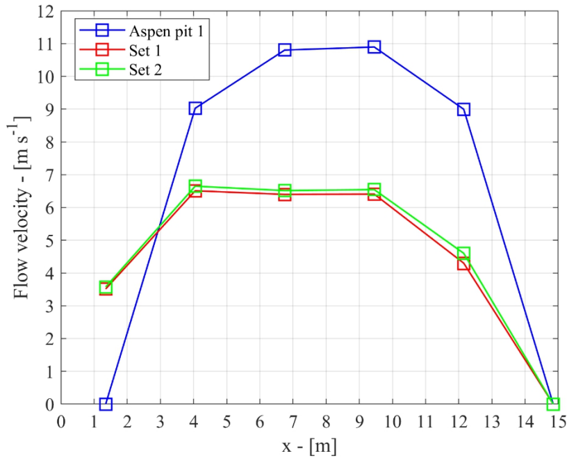
395 Figure 12. Peak flow velocity module at the measuring cross-section. Aspen pit 1 rheological set is given by C_v = 0.313 , \alpha_1 = 0.0036 \text{ Pa s} , \alpha_2 = 0.0181 \text{ Pa} , \beta_1 = 22.1 , \beta_2 = 25.7 , \gamma_m = 26.5 \text{ kN m}^{-3} , n = 0.1 \text{ s m}^{-1/3} and K = 2285 . Rheological set 1 is given by C_v = 0.423 , \alpha_1 = 0.0036 \text{ Pa s} , \alpha_2 = 0.0181 \text{ Pa} , \beta_1 = 20.5 , \beta_2 = 25.7 , \gamma_m = 26.5 \text{ kN m}^{-3} , n = 0.1 \text{ s m}^{-1/3} and K = 2285 . Rheological set 2 is given by C_v = 0.423 , \alpha_1 = 0.0036 \text{ Pa s} , \alpha_2 = 0.001 \text{ Pa} , \beta_1 = 20.5 , \beta_2 = 25.7 , \gamma_m = 26.5 \text{ kN m}^{-3} , n = 0.1 \text{ s m}^{-1/3} and K = 2285 .
