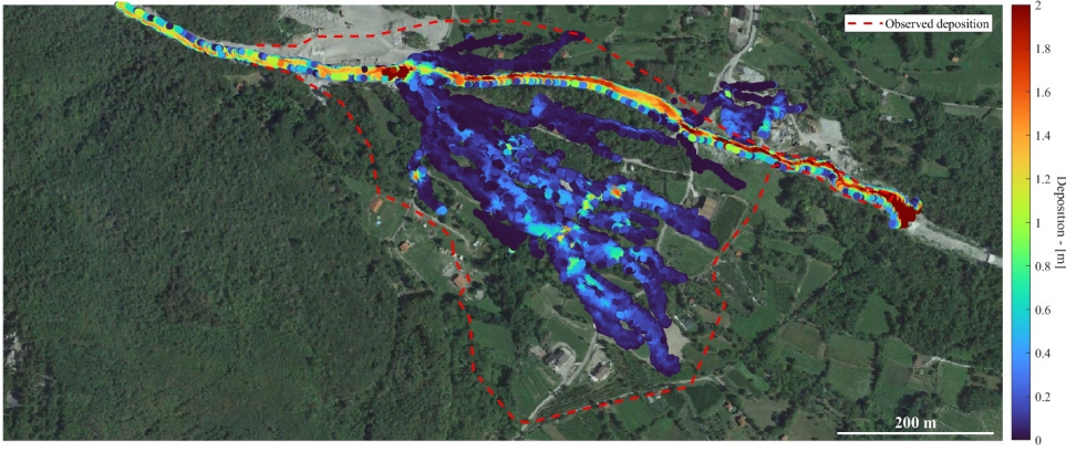
Figure 11. Deposition map at the end of the simulation using the O'Brien model with C_v = 0.423, \alpha_1 = 0.0036 \text{ Pa s}, \alpha_2 = 0.001 \text{ Pa}, \beta_1 = 20.5, \beta_2 = 25.7, \gamma_m = 26.5 \text{ kN m}^{-3}, n = 0.1 \text{ s m}^{-1/3} and K = 2285 (© Google Earth 2019).
