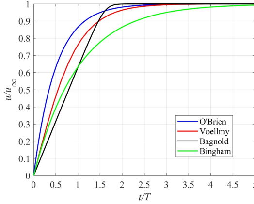
Figure 1. Dimensionless analytical solution for 4 different rheological models. The solution (5) using the O’Brien rheology is shown in blue using the ‘‘Aspen Pit 1’’ parameters set with \gamma_w = 9\,810 \text{ N m}^{-3} (water specific weight), \gamma_s = 26\,500 \text{ N m}^{-3} (specific weight of sediments), n = 0.033 \text{ s m}^{-1/3} and K = 2285 . The solid red line is the analytical solution (17) for the Voellmy rheology using \mu = 0.1 and \xi = 1000 \text{ m s}^{-2} . The solid green line shows the solution computed using Bingham frictional law (21) with \tau_c = 200 \text{ Pa} , \gamma_m = 15\,000 \text{ N m}^{-3} and \eta = 90 \text{ Pa s} . Finally the black line is the numerical solution using Bagnold frictional law with \rho_s = 2\,300 \text{ kg m}^{-3} , \rho_w = 1\,000 \text{ kg m}^{-3} , \phi_d = 35^\circ , Y = 40 , \beta = 1 and c_b = 0.65 . In this case, being a numerical solution, there is no formula for the characteristic time, and the time at which the flow reaches 63% of the uniform velocity has been arbitrarily selected as the characteristic time for the normalization. In all cases the debris flow layer h is equal to 1 \text{ m} and the channel slope is 20^\circ .
