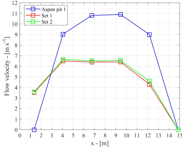
Figure 12. Peak flow velocity module at the measuring cross-section. Aspen pit 1 rheological set is given by C_v = 0.313, \alpha_1 = 0.0036 \text{ Pa s}, \alpha_2 = 0.0181 \text{ Pa}, \beta_1 = 22.1, \beta_2 = 25.7, \gamma_m = 26.5 \text{ kN m}^{-3}, n = 0.1 \text{ s m}^{-1/3} and K = 2285 . Rheological set 1 is given by C_v = 0.423, \alpha_1 = 0.0036 \text{ Pa s}, \alpha_2 = 0.0181 \text{ Pa}, \beta_1 = 20.5, \beta_2 = 25.7, \gamma_m = 26.5 \text{ kN m}^{-3}, n = 0.1 \text{ s m}^{-1/3} and K = 2285 . Rheological set 2 is given by C_v = 0.423, \alpha_1 = 0.0036 \text{ Pa s}, \alpha_2 = 0.001 \text{ Pa}, \beta_1 = 20.5, \beta_2 = 25.7, \gamma_m = 26.5 \text{ kN m}^{-3}, n = 0.1 \text{ s m}^{-1/3} and K = 2285 .
