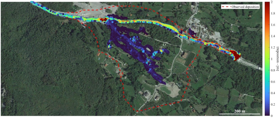
390 Figure 10. Deposition map at the end of the simulation using the O'Brien model with C_v = 0.423 , \alpha_1 = 0.0036 \text{ Pa s} , \alpha_2 = 0.0181 \text{ Pa} , \beta_1 = 20.5 , \beta_2 = 25.7 , \gamma_m = 26.5 \text{ kN m}^{-3} , n = 0.1 \text{ s m}^{-1/3} and K = 2285 (© Google Earth 2019).
