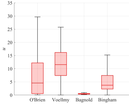
Figure 2. Uniform velocity boxplot distribution for the 4 rheological models used to perform Sobol sensitivity analysis ( h = 1 m, \theta = 20^\circ ). For each graph the solid line represents the median value across the whole distribution, the rectangular box covers the range from the lower quartile (25%) to the upper quartile (75%) and the whiskers show the non-outlier maximum (the maximum data value which is not an outlier) and minimum (the minimum data value which is not an outlier). Here a point is classified as an outlier if it lies more than 1.5 times the interquartile range away from the top or bottom of the red-shaded rectangle.
