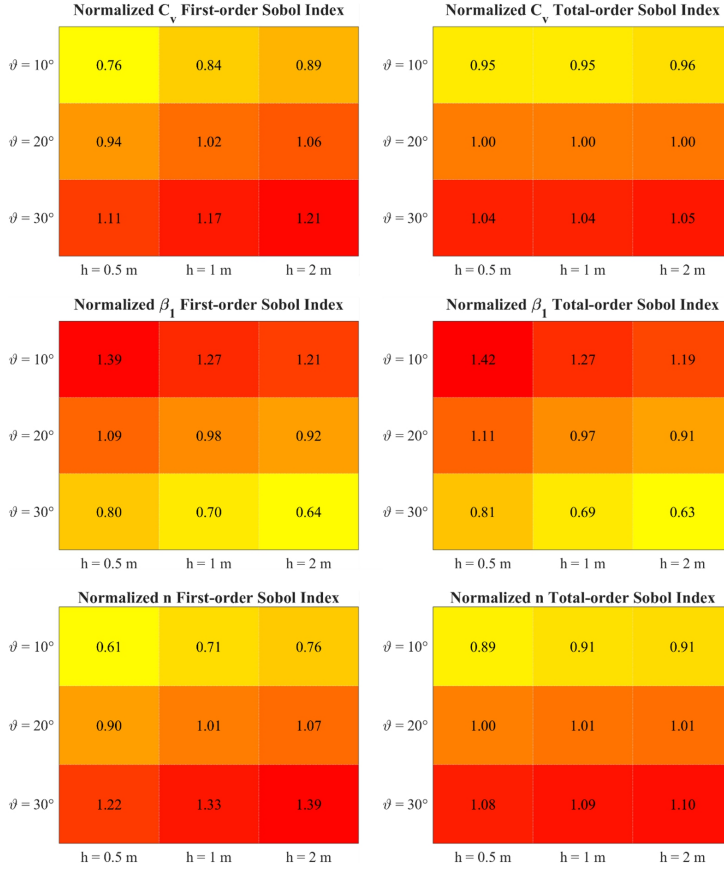
Figure 4. First-order (left) and total-order (right) Sobol' index for the parameters C_v , \beta_1 and n as a function of different values of \vartheta and h . Each entry of the matrix represents the first- (total-) order Sobol' index computed using the corresponding (h, \vartheta) couple, then divided by the average index over the whole matrix. The average first-order (total-order) Sobol' indices for C_v , \beta_1 and n are 0.34 (0.6), 0.19 (0.41) and 0.13 (0.38) respectively.
